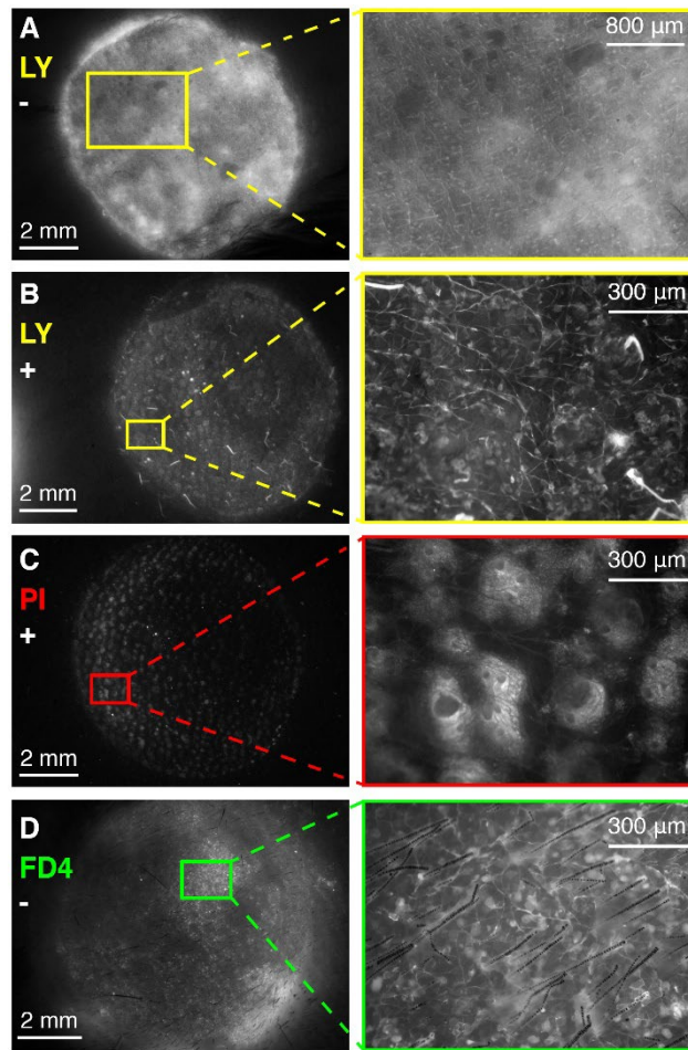
Fig. 7. Molecular delivery into skin model after PEF at 300 V. Images showing the patterns of fluorescence with (A) Lucifer Yellow (LY) under negative electrode with optical zoom of 1.25x (left) and 3.2x (right); (B) LY under positive electrode with optical zoom of 1.25x (left) and 9.2x (right); (C) Propidium Iodide (PI) under positive electrode with optical zoom of 1.25x (left) and 9.2x (right); (D) Fluorescein isothiocyanate–dextran under negative electrode with optical zoom of 1.25x (left) and 9.2x (right). LY fluorescence mostly originates from the paracellular space of the stratum corneum (B), while Propidium Iodide is located in the intracellular space of nucleated cells, in the viable skin (C). Brightness and contrast are customized for each capture.
