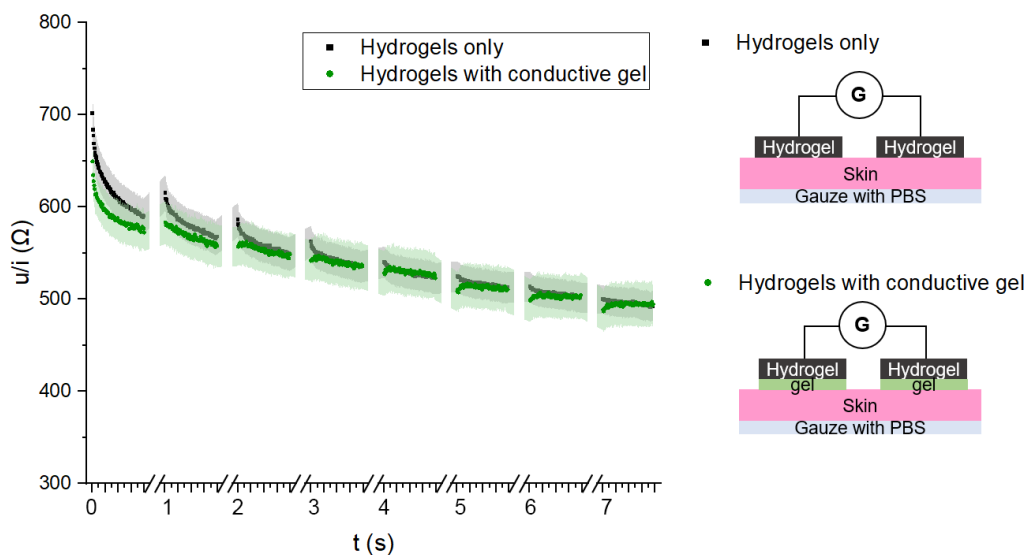
Fig. S3. Instantaneous resistance ( r(t)=u(t)/i(t) ) of electroperoration system with skin and hydrogels only (black, n=12 ) and with skin, hydrogels and conductive gel between them (green, n=3 ). Adding conductive gel between the hydrogels and the skin does not improve electrical contact, therefore it is rendered unnecessary, for our configuration. Shaded areas represent SEM.
