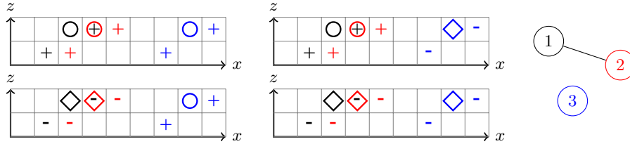
Fig. 5. Parity planes and \theta -effect planes of four parity-bare states that are scalar-equivalent and their associated graph.
