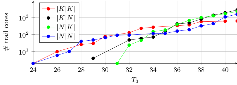
Fig. 8. Number of 3-round trail cores of weight W such that |W| \leq T_3 for different parity profiles.
