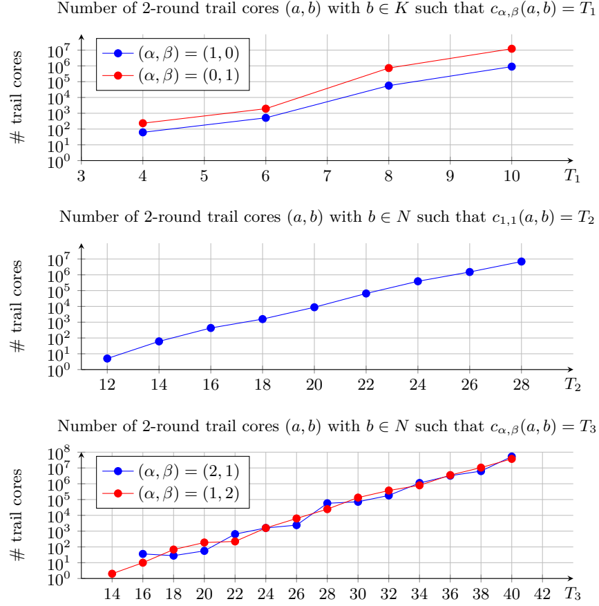
Fig. 7. Number of 2-round trail cores for different cost functions. Trail cores are considered in the three graphs up to z-invariance. In the second graph, trail cores are also considered up to scalar-equivalence.
