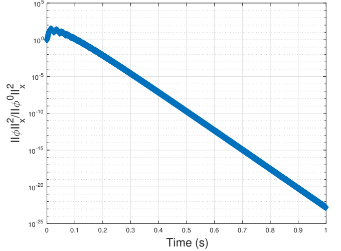
Fig. 4. Time evolution of \frac{\|\phi\|_x^2}{\|\phi^0\|_x^2} in logarithmic scale
