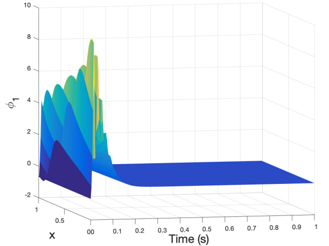
Fig. 1. State \phi_1 over (t,x) plane, (final time T = 1s )
