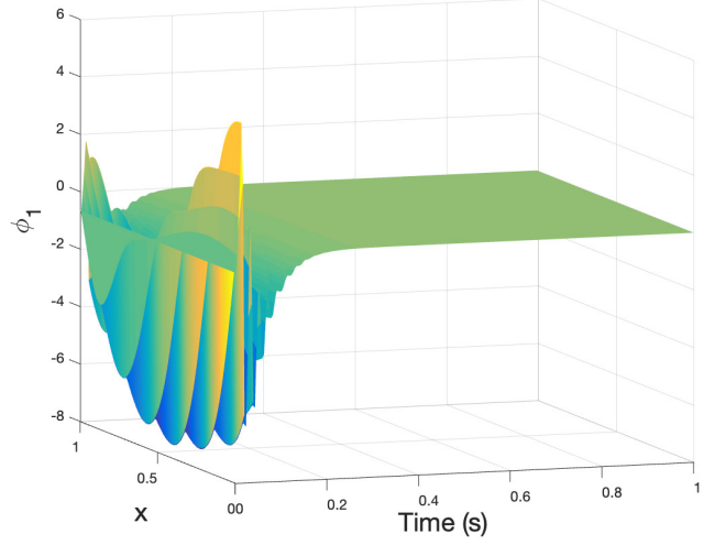
Fig. 3. State \phi_1 over (t,x) plane, (final time T = 1 s)
