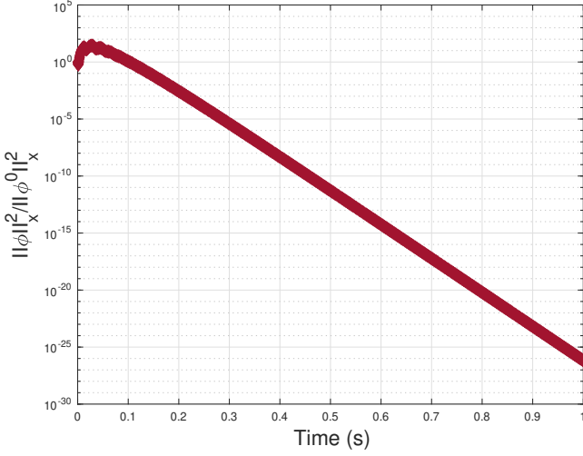
Fig. 2. Time evolution of \frac{\|\phi\|_x^2}{\|\phi^0\|_x^2} in logarithmic scale
