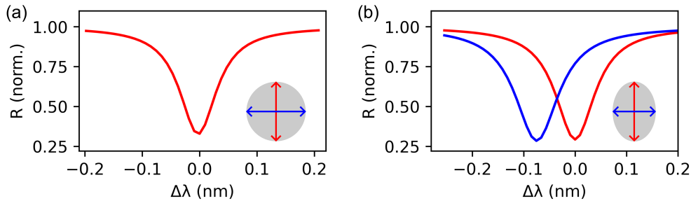
Figure 1. Fitted reflectivity spectra of a (a) circular micropillar with a diameter of 4\ \mu\text{m} and (b) an elliptical micropillar with a major (minor) axis length of 4\ \mu\text{m} ( 2.4\ \mu\text{m} ).
