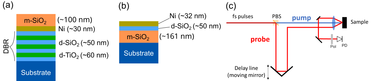
Figure 1. (a-b) Multilayer structure schematics of the (a) top-cavity acoustic resonator and (b) reference sample. (c) Schematics of the pump-probe experiment. PBS, Pol and PD stand for polarizing beam splitter, polarizer and photodetector, respectively.
