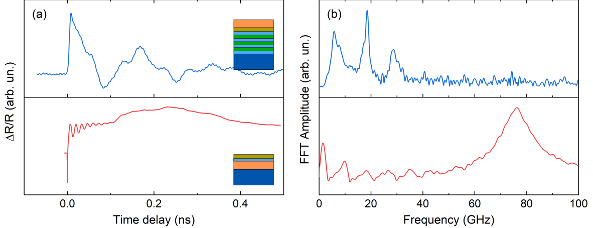
Figure 2. (a) Reflectivity time trace of the acoustic resonators. Top and bottom panels correspond to the measurements performed on the top-cavity and reference resonator, respectively. (b) Fourier transform of the respective time traces displayed in (a).
