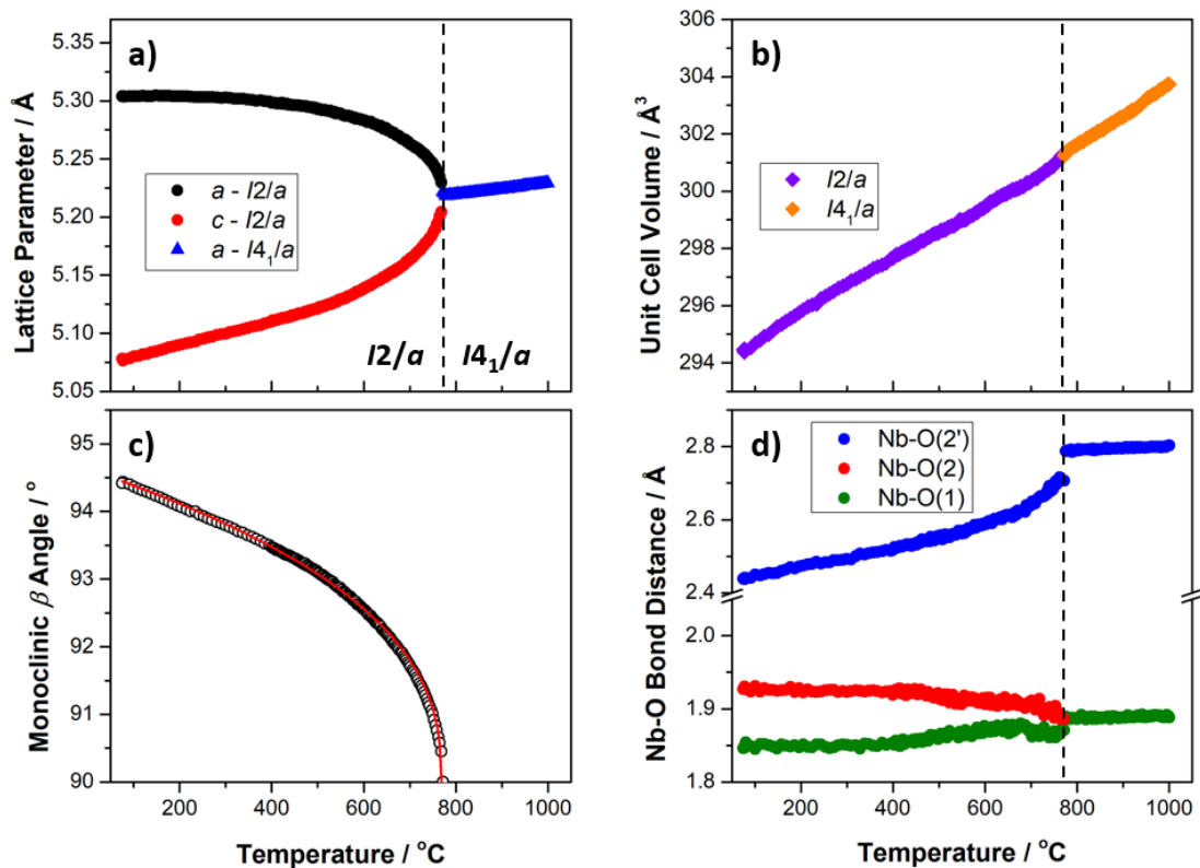
Figure 4: Temperature dependence of the unit cell parameters for \text{HoNbO}_4 obtained by Rietveld refinements against neutron powder diffraction data. The data were collected as the sample was heated from room temperature to 1000 °C. The error bars are smaller than the symbols. The solid line in © is a fit described in the text.
