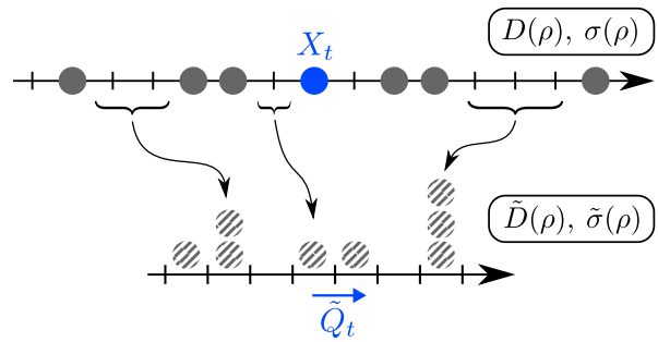
FIG. 1. An example of mapping between two single-file systems. The SEP (top) is mapped onto a zero range process (ZRP, below). This well-known mapping holds at the microscopic level: the empty sites of the SEP becomes the particles of the ZRP [2], while the position X_t of the tracer in the SEP is mapped onto the integrated current through the origin \tilde{Q}_t in the ZRP. At the macroscopic level, such a mapping holds for any single-file system [30]: the tracer in a system with transport coefficient D(\rho) and \sigma(\rho) is mapped onto the current in a system with \tilde{D}(\rho) and \tilde{\sigma}(\rho) given by (3).
