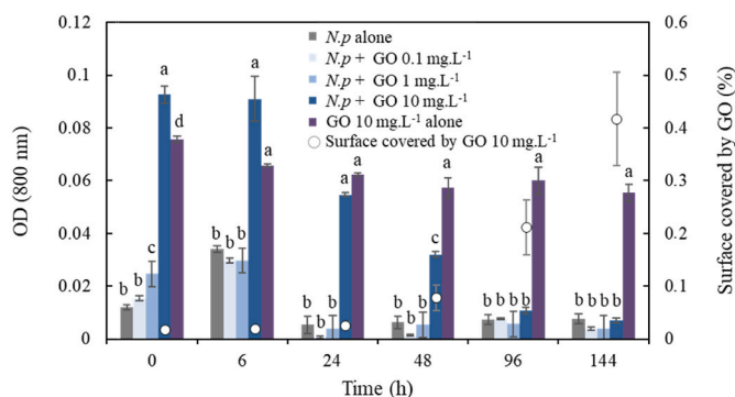
Fig. 7. Sticking of GO by Nitzschia palea through time. Bar charts represents the OD at 800 nm of the water column as a function of time. The dots represent the percentage of surface covered by GO at the bottom of the well during the exposure at 10 \text{ mg L}^{-1} . Letters correspond to significantly different groups at each sampling time (TukeyHSD p < 0.05 ).
