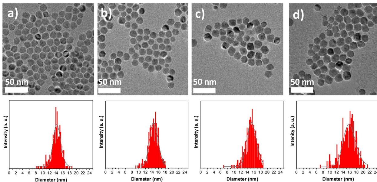
Fig. 2 TEM images of (a) CS, (b) CSSa, (c) CSSb, and (d) CSSc and the corresponding size distributions (bottom).
