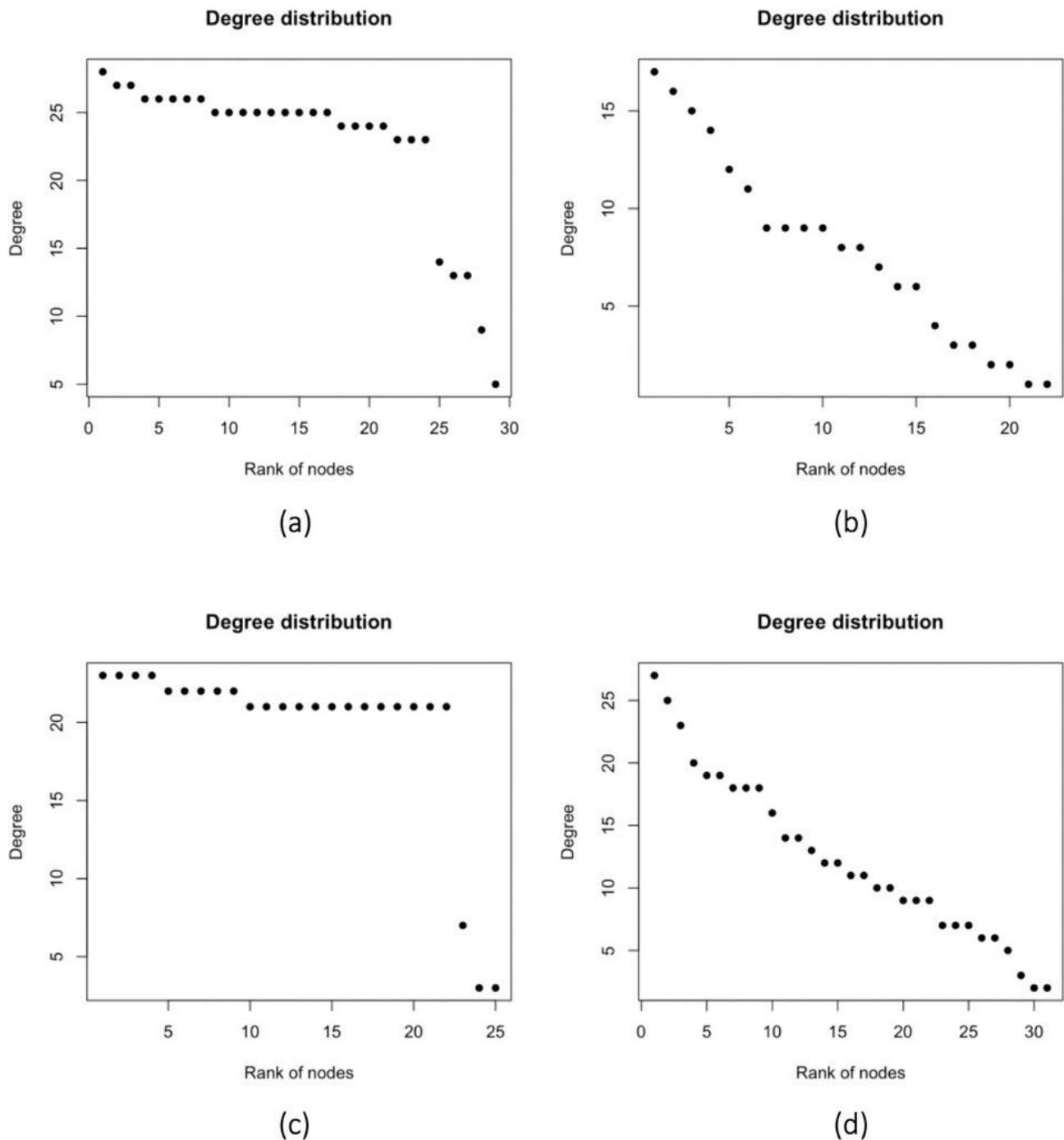
Figure 5. Degree distribution for each phase.
