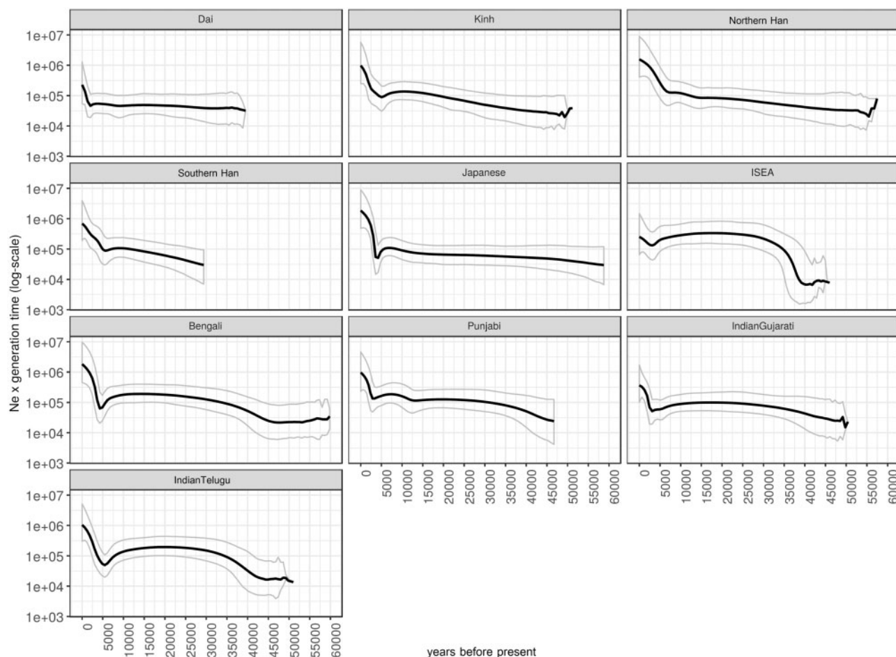
FIG. 7. The BSPs of Asian populations. Solid lines are the median estimated paternal effective population size ( y axis) through time from the present in years ( x axis). The 95% highest posterior density limits are indicated by dotted lines.
