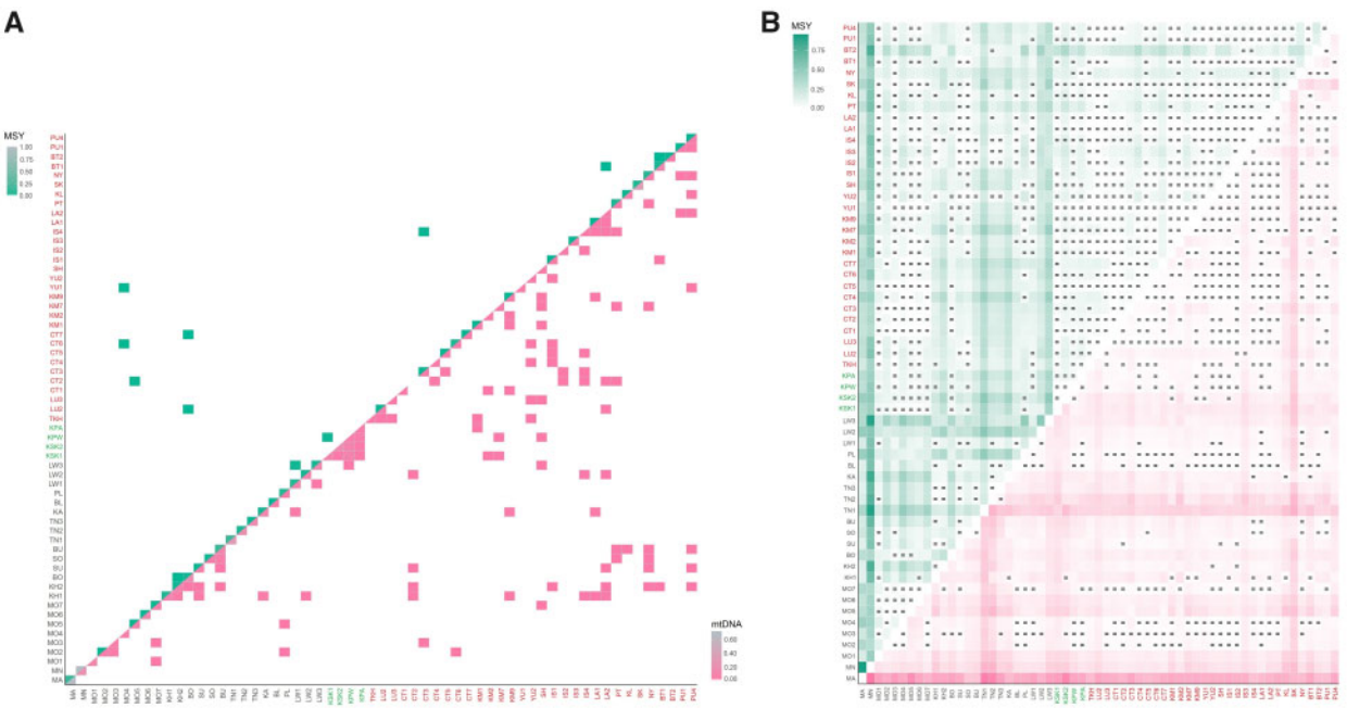
FIG. 3. Relative shared haplotypes (A) and heat plot of \Phi_{st} (B) between studied populations for the MSY and for mtDNA.
