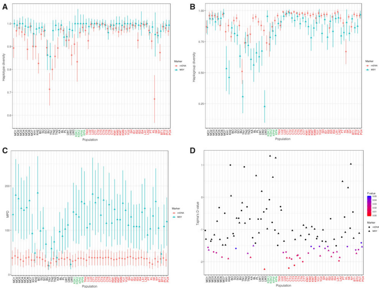
FIG. 2. Genetic diversity values of MSY and mtDNA in the studied populations, excluding the Maniq (MN) and Mlabri (MA): haplotype diversity (A), haplogroup diversity (B), MPD (C), and Tajima's D values (D). More information and all genetic diversity values are provided in supplementary table 1, Supplementary Material online.
