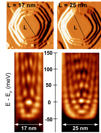
FIG. 1 (color online). Topographic STM image of a truncated hexagonal Ag pyramid and spectroscopic map obtained from 64 dI/dV spectra recorded along the line of the topographic images. It evidences the localization of the confined states in the hexagonal surface.
