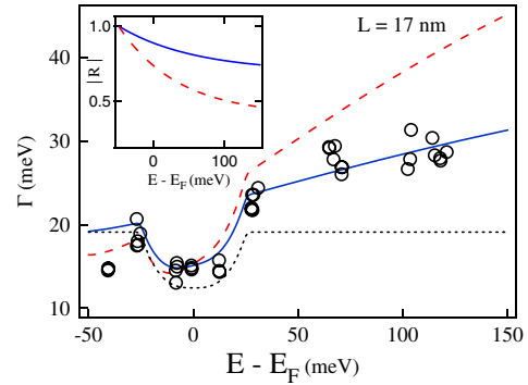
FIG. 3 (color online). Experimental spectral width of the confined states of a 17 nm pyramid (symbols). The dotted black line shows the electron-phonon scattering contribution calculated in a simple Debye model with \omega_D = 25 meV, \lambda = 0.12 , and T = 5 K. The dashed (red) and solid (blue) lines represent the sum of the contribution of the electron-phonon interaction and lossy boundary contributions calculated with the step and quasi-ideal coefficients, respectively. These three curves have been shifted by the defect contribution (12 meV). Inset: quasi-ideal resonator (solid blue line) and step (dashed red line) reflection coefficients.
