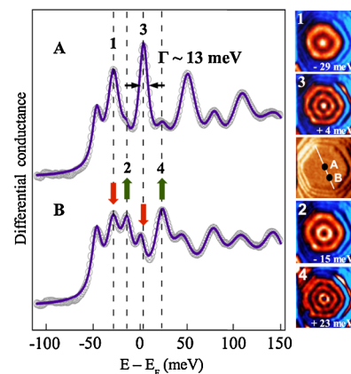
FIG. 2 (color online). dI/dV spectra recorded in the A and B points in the topographic STM image reported in the right part. The solid black line represents the fitting curve composed of Lorentzian structures associated with the confined states. In the right part, dI/dV maps are shown corresponding to the 1–4 energy, as well as a STM image showing the position of the A and B points.
