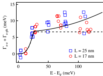
FIG. 4 (color online). Intrinsic linewidth as a function of energy for the confined states. Circles and squares correspond to the value for two different pyramid sizes L = 17 nm and L = 25 nm. The dotted line represents the electron-phonon contribution; the solid line represents the sum with the electron-electron contribution. The defect contributions are 10.7 meV and 8.5 meV for the 17 nm and 25 nm pyramids, respectively.
