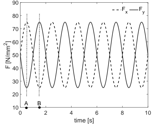
(b) Time evolution of prescribed external forces. Highlight of time instants A ( t = 0.5 s) and B ( t = 1.5 s).
