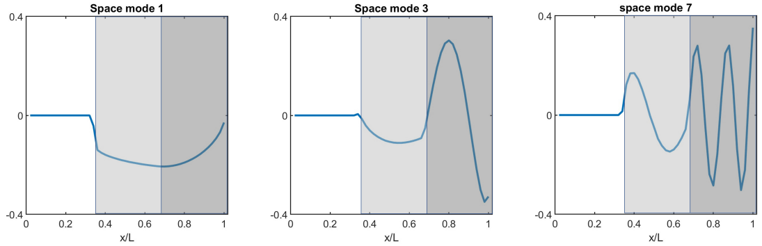
Figure 4: SVD space modes 1, 3 and 7 of the frictional contact forces. The corresponding singular values are 6.27 \cdot 10^4 , 1.55 \cdot 10^4 , and 5.77 \cdot 10^3 .
