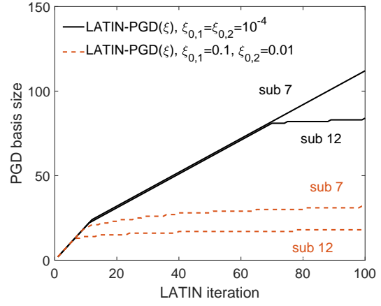
(b) PGD basis size along the iterations for the LATIN-PGD( \xi ) strategy.
