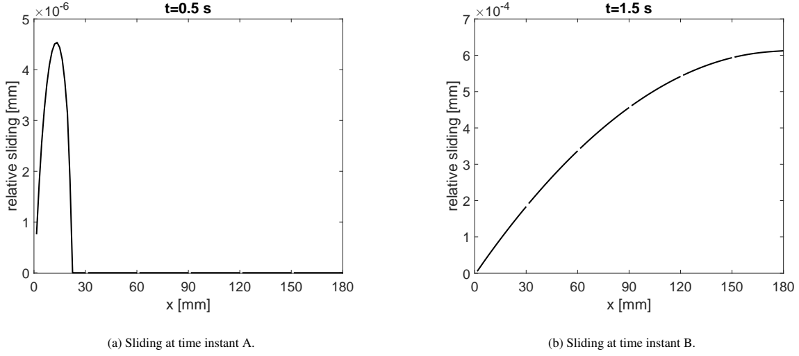
Figure 23: Relative sliding along the contact interface \Gamma_c at time instants A and B.
