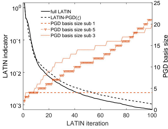
(a) LATIN indicator and PGD basis size per substructure.
