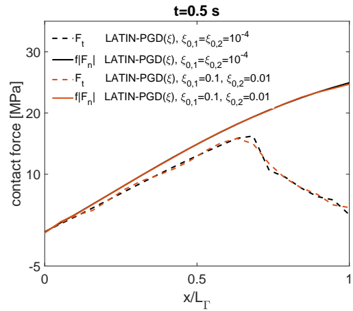
(b) Linear stage normal and tangential forces at iteration 500.
