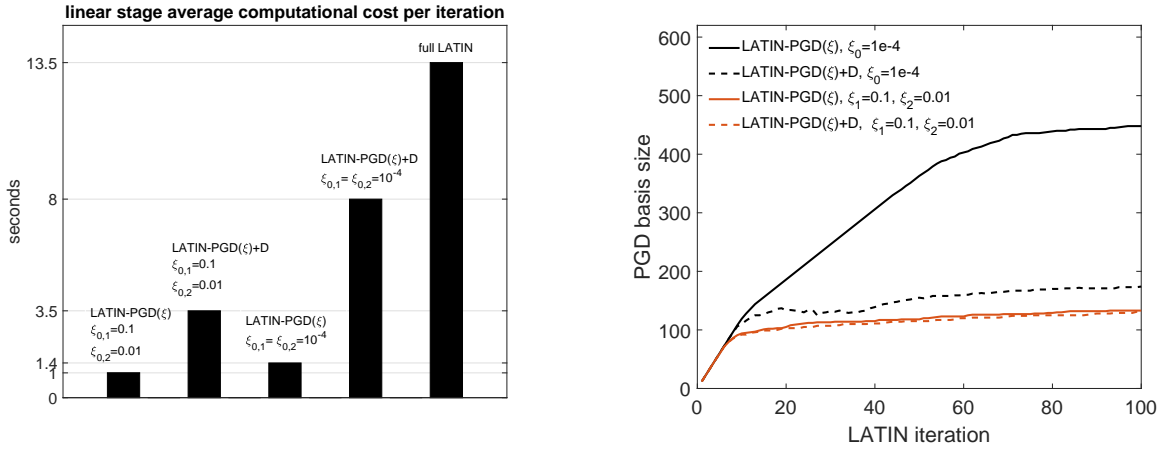
(a) Computational cost of the linear stage of the LATIN-PGD( \xi ), LATIN-PGD( \xi )+D and full LATIN. (b) PGD basis size of LATIN-PGD( \xi ) and LATIN-PGD( \xi )+D for substructures 7 to 12.
