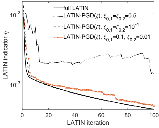
(a) LATIN convergence indicator of full LATIN and LATIN-PGD( \xi ).
