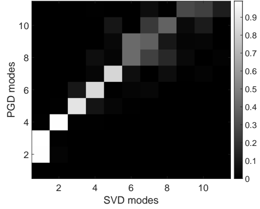
(b) MAC diagram for mixed modes \{L_k\} of substructure 5.
