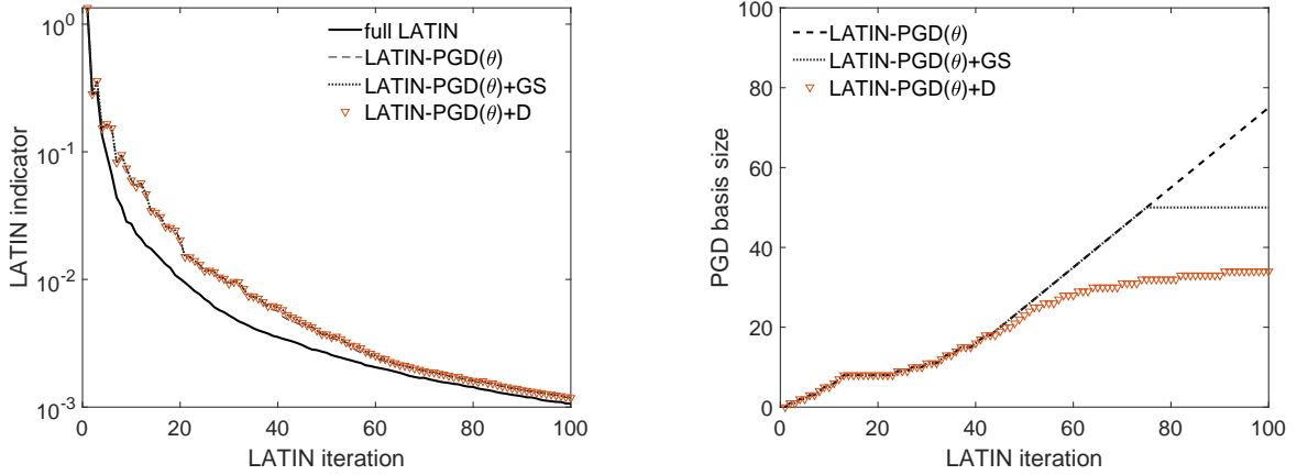
(a) LATIN convergence indicator for full LATIN, LATIN-PGD( \theta ), LATIN-PGD( \theta )+GS and LATIN-PGD( \theta )+D. (b) Basis size along the LATIN iterations of the LATIN-PGD( \theta ), LATIN-PGD( \theta )+GS and LATIN-PGD( \theta )+D.
