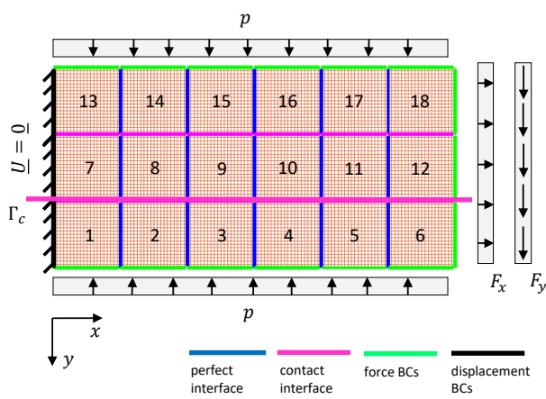
(a) Representation of substructures and interfaces, with numbering of the substructure. Highlight of the contact interface \Gamma_c between two beams.
