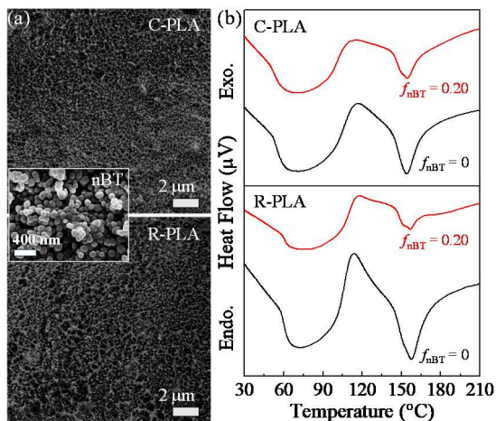
Fig. 1 (a) SEM images of nBT nanoparticles and the fractured surfaces of C-PLA/nBT and R-PLA/nBT nanocomposites with f_{\text{nBT}} = 0.20 . (b) DTA curves of C-PLA/nBT and R-PLA/nBT nanocomposites with f_{\text{nBT}} = 0 and 0.20.
