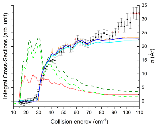
Fig. 13 Experimental and theoretical cross-sections for the HDO + normal -H 2 → HDO ( 1_{01} or 1_{11} ) + H 2 inelastic collisions. Squares are experimental ICSs for the 1_{11} rotational level, with error bars corresponding to statistical uncertainties at 95% of the confidence interval (a square represents the mean of around 5000 data). Shown as solid lines, the total theoretical contributions are convoluted to the experimental collision-energy spread assuming an initial rotational population from the 1_{01} state of 5% (as a bold cyan line) or 0% (as a bold blue line), with partial contributions of the 1_{11} \leftarrow 0_{00} transition (as an orange line) and the 1_{11} \leftarrow 0_{01} transition (as a red line). Shown as dashed lines, the simulated total theoretical contributions are convoluted to the experimental collision-energy spread for the 1_{01} rotational level, assuming an initial rotational population from the 1_{01} state of 5% (in green) or 0% (in olive), as done for the HDO + Ne system.
