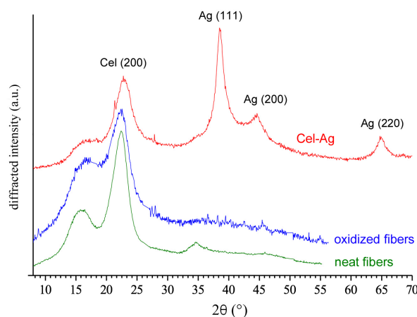
Fig. 2: XRD profiles of neat cellulose fibers (green), \text{NaIO}_4 -oxidized fibers (blue), and hybrid Cel-Ag nanofibrils after Tollens' reaction (red).
