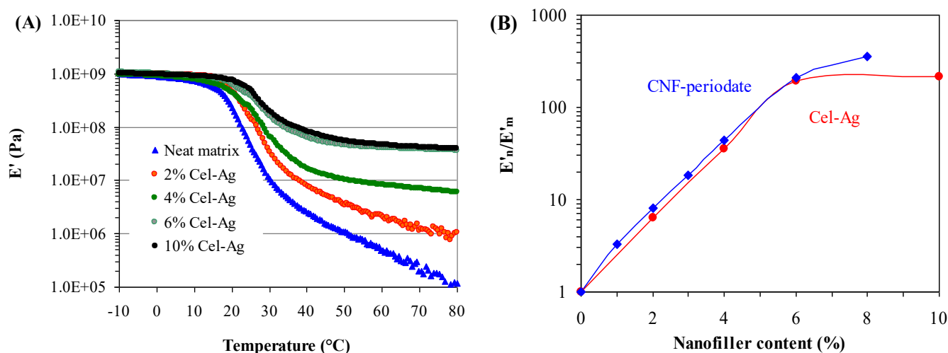
Fig. 6: (A) Storage tensile modulus, E' , vs. temperature at 1 Hz and (B) evolution of the increment in modulus vs. Cel-Ag content at 70 °C.
