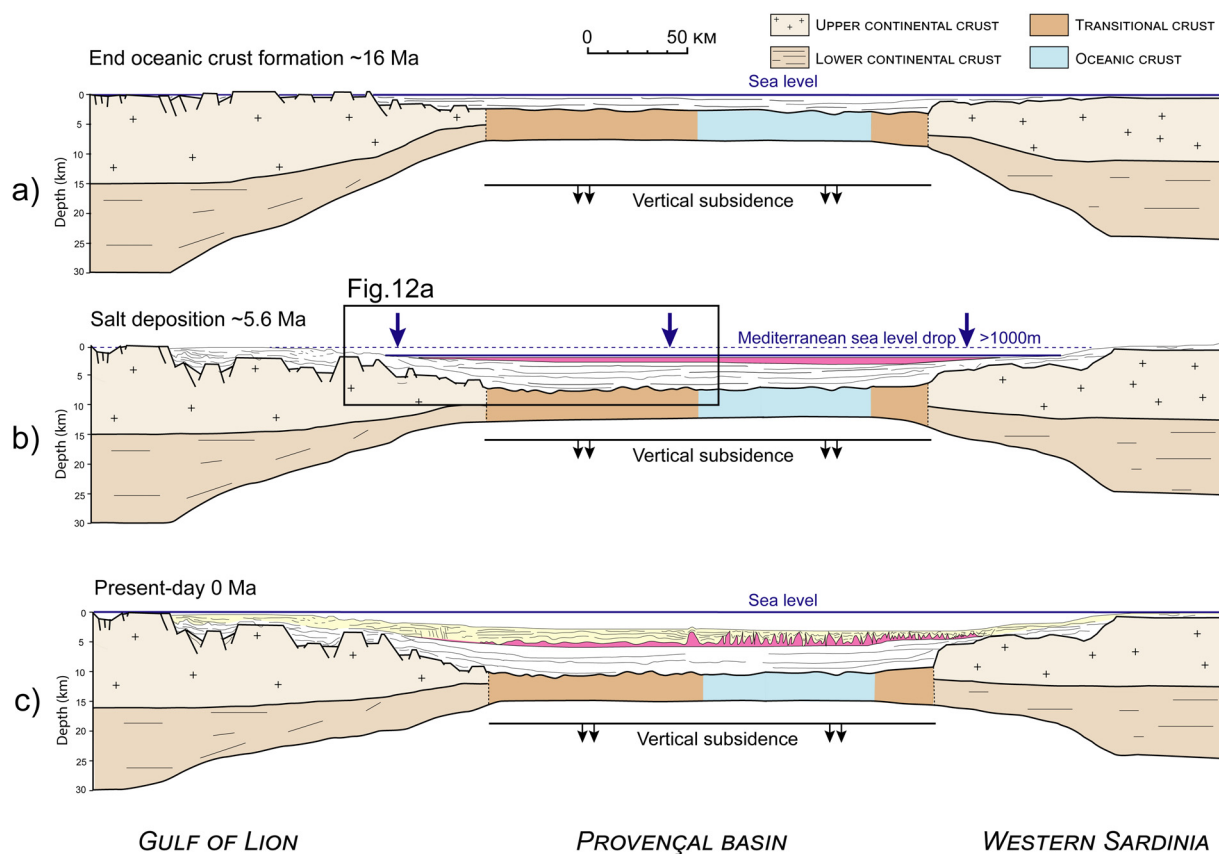
Fig. 4. Sketch illustrating the Messinian salt deposition compared to the subsidence evolution in the Gulf of Lion, Provençal Basin and Western Sardinian conjugated margins. (a) Basin reconstruction at 16 Ma: the Corso-Sardinian block ceased the counter-clockwise rotation; the deep basin, composed by proto-oceanic crust and bordered by transitional crust, (Moulin et al. , 2015; Afilhado et al. , 2015) is characterized by a vertical subsidence. (b) Basin reconstruction at ~5.6 Ma: the Messinian sea-level drop took place leading to the salt deposition above a thick pre-salt sequence. The initial salt thickness is considered constant except on the margin edges. (c) Basin reconstruction at present-day: after the reflooding and the end of the MSC (5.32 Ma) the Pliocene-Pleistocene sedimentation filled the basin and margins. Wide variations in salt morphologies are observed at present-day.
