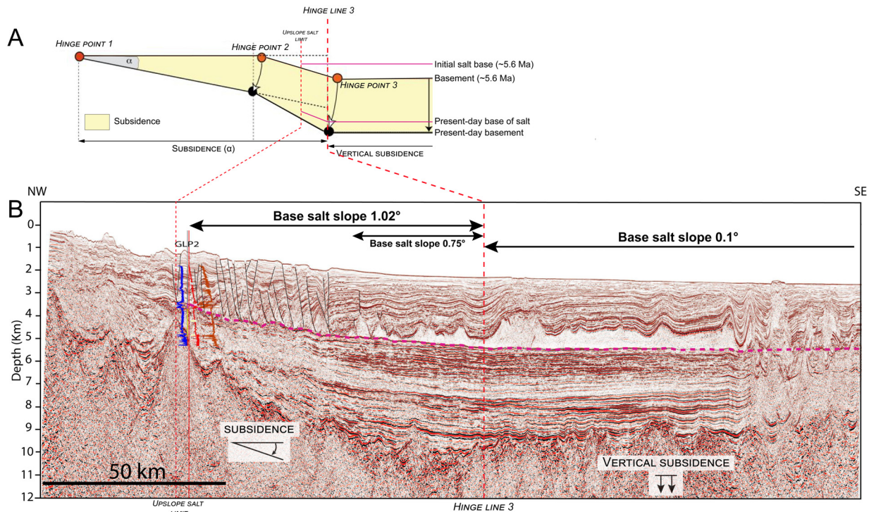
Fig. 2. (A) Sketch illustrating how has been analysed the subsidence pattern of the Provençal Basin (modified after Leroux, 2012). Hinge line 3 marks the boundary between a tilting and purely vertical subsidence. Dotted black lines highlight the slope changing basinward the hinge points. Note the increasing slope history on the margin given by subsidence while the deep basin subsides purely vertically. (B) Seismic profile (in depth, km) (TGS-Nopec) crossing perpendicularly the Provençal Basin (location in Fig. 1) showing the base of salt slope values (dashed purple line) in the lower slope and deep basin. The profile is modified from Bache et al. , 2015. Vertical exaggeration \times 6 .
