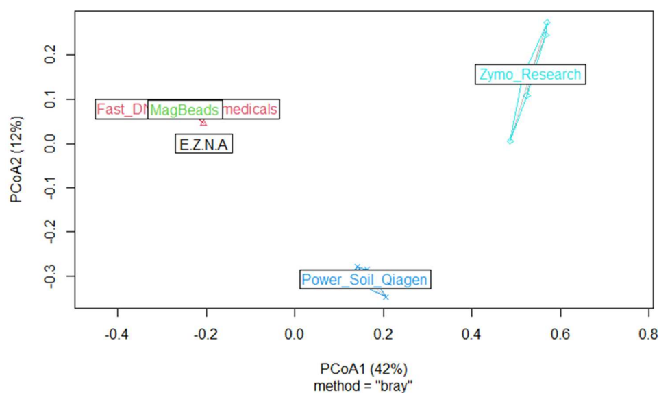
Figure 8. PCoA-bacteria-Data: Multidimensional scaling plots based on the Bray–Curtis distance and reflecting differences in the beta microbial diversity community composition of the five kits.
