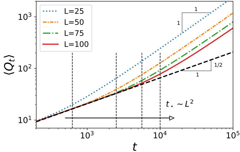
FIG. S1. Mean integrated current \langle Q_t \rangle for a finite system of length L , connected to reservoirs at densities \rho_L = 0.75 and \rho_R = \bar{\rho} = 0.16 , obtained from (S12-S14), for different system sizes. In a first regime, the mean current follows the predicted behavior for a semi-infinite system (black dashed line). After a crossover time t_* , which scales as L^2 , the mean current grows linearly with time, indicating that the system has reached a steady state.
