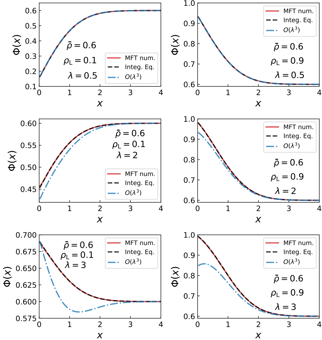
FIG. S2. Numerical solution of the MFT equations (S21-S24) (solid red line), compared to the solution of the integral equation (S71), together with the boundary conditions (S10,S11) (dashed black line) and the solution up to order 3 in \lambda given by (S61-S63) (dotted blue line). Left: for \bar{\rho} = 0.6 , \rho_L = 0.1 . Right: for \bar{\rho} = 0.6 , \rho_L = 0.9 . Top: \lambda = 0.5 . Middle: \lambda = 2 . Bottom: \lambda = 3 .
