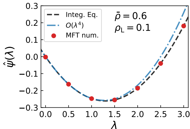
FIG. S3. Cumulant generating function \hat{\psi}(\lambda) as a function of \lambda , for \bar{\rho} = 0.6 and \rho_L = 0.1 . The red points are obtained from the numerical resolution of the MFT equations (S21-S24). The dashed black line corresponds to our result (S80), which results from the closed integral equation (S71). The dotted blue line corresponds to the first three orders in \lambda , given in (S64).
