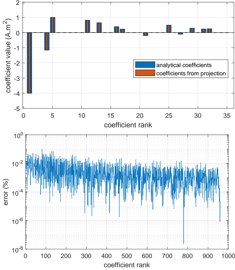
Figure 10: Two sets of normalized spherical harmonic coefficients \bar{a}_{km} for the first five orders (above) and relative difference \varepsilon between them (below).
