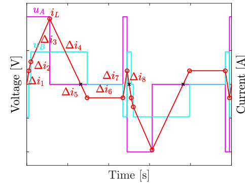
(f) DAB ZVS Trapezoidal 3 (novel)
