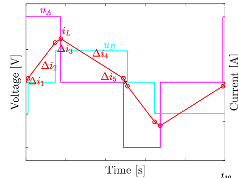
(h) DAB ZVS Trapezoidal 1 (TPS modulation)
