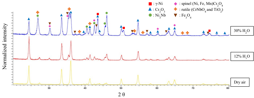
Fig. 4 Comparison of low-incidence ( 5^\circ ) XRD analysis in the center zone of upstream In625 samples oxidized for 400 h at 900^\circ\text{C} and under \text{N}_2\text{-O}_2\text{-X}\%\text{H}_2\text{O} (vol. %)
