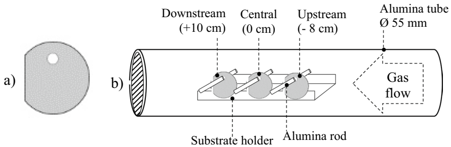
Fig. 1 a Sample scheme and b sample positioning within the furnace of the high-temperature oxidation rig
