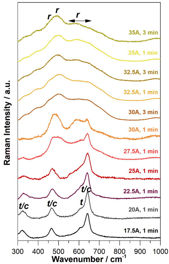
Figure 5. Raman spectra of samples sintered under N 2 atmosphere. The peaks are indexed as follows: c = cubic, t = tetragonal YSZ, r = rock salt.
