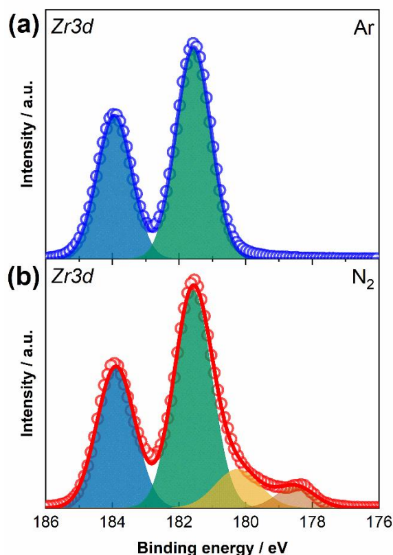
Figure 8. XPS spectrum of Zr3d for samples sintered at 30 A for 1 min in (a) Ar and (b) N 2 .
