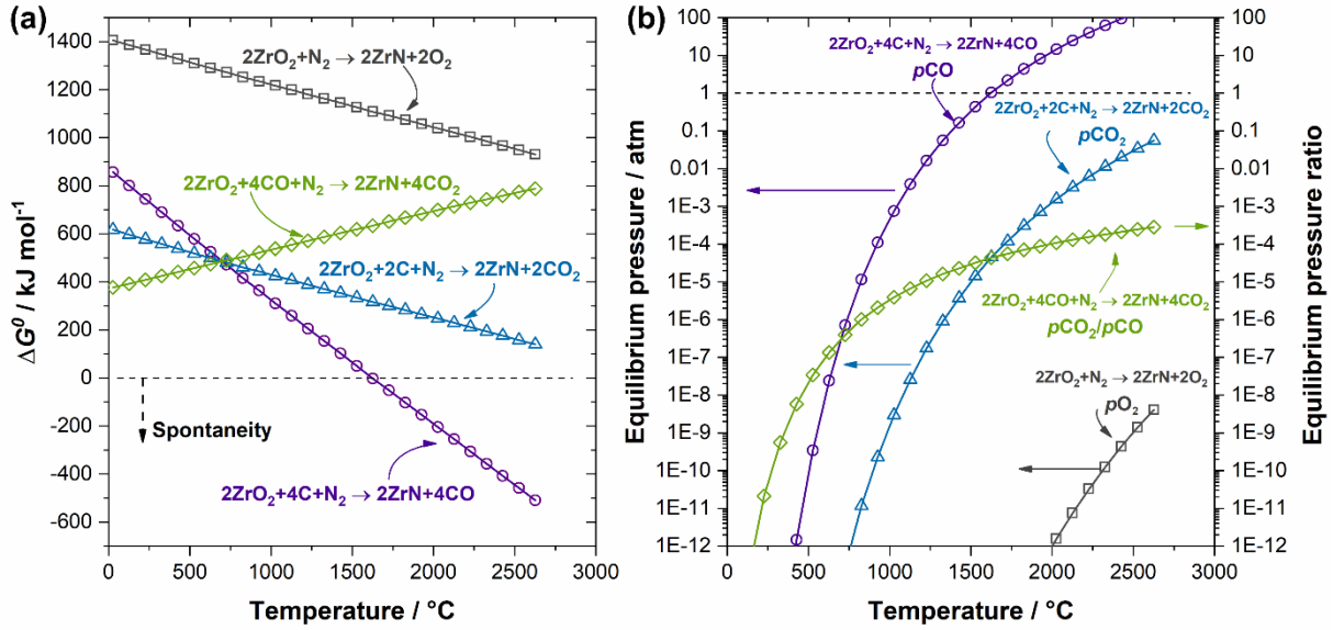
Figure 12. a) Standard Gibbs free energy change associated to different possible reaction leading to the formation of ZrN in UHS; b) partial pressure of the different gasses at the equilibrium calculated using Eq 12-15 . Thermochemical data taken from [81].
