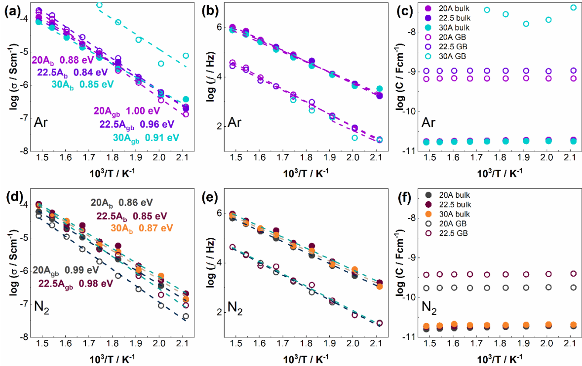
Figure 11. Data obtained from EIS measurements fits for samples produced in (a-c) Ar and (d-f) N 2 (a, d) conductivity, (b, e) relaxation frequency (c, f) equivalent capacitance.
