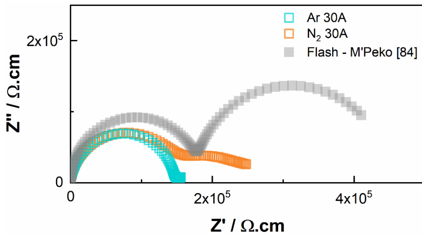
Figure 10. Nyquist plot for impedance data of UHS sintered samples at 30A in Ar and N_2 and data obtained by M'Peko et al. in Flash Sintering of 3YSZ at 900^\circ\text{C} -1A-60s [84].
