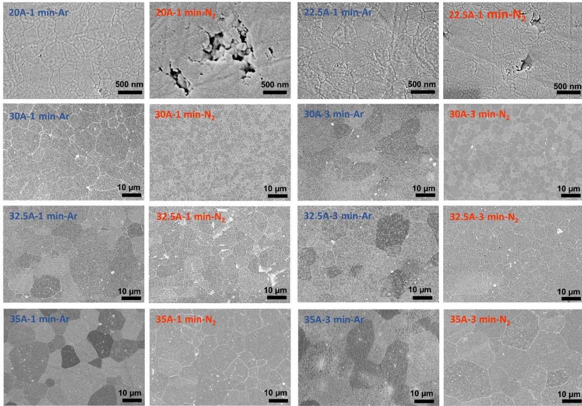
Figure 2. SEM micrographs of polished cross-sections of the samples produced under different currents (A), dwell time (min), and environmental conditions (Ar or N 2 ).
