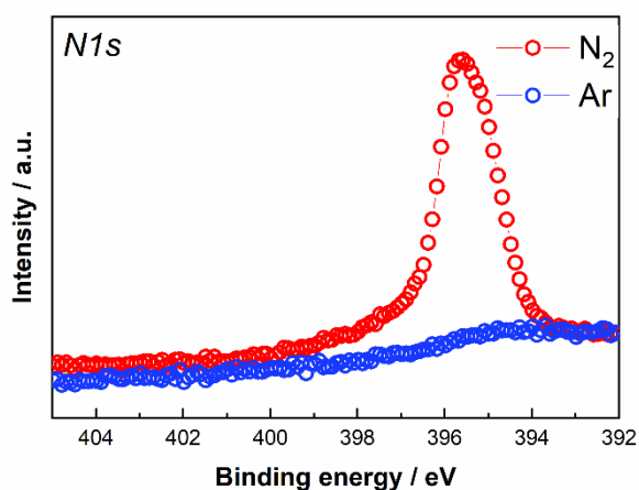
Figure 7. XPS spectrum of N1s for samples sintered in Ar and N 2 at 30 A – 1 min.
