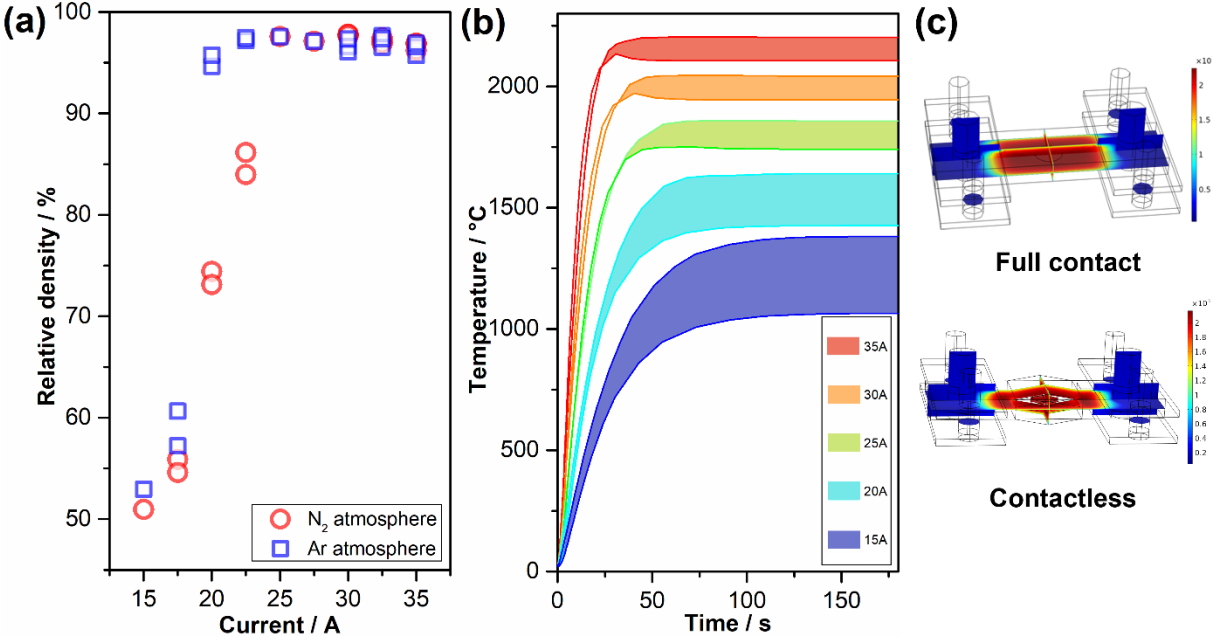
Figure 1. (a) Relative density of 3YSZ samples treated under Ar and N 2 atmosphere as a function of current (each single point corresponds to a different sample); (b) simulation of the temperature range evolution upon UHS at different applied currents. The highest temperature is simulated by the Fem full-contact configuration and the lowest one by the contactless as reported in (c). Details about FEM are available in ref [30]. The relative density was calculated assuming the density of YSZ constant (6.05 g cm -3 ).
