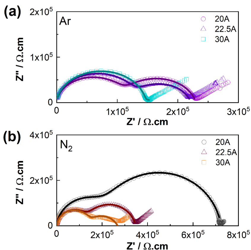
Figure 9. Nyquist plot of complex impedance (300°C) of samples sintered under different currents in (a) Ar and (b) N_2 . The fitting is represented by the solid lines.
