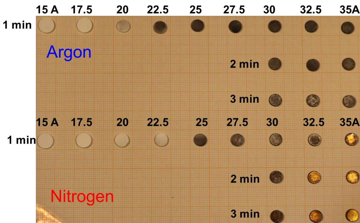
Figure 6. Image of the samples under different current, time, and atmospheric (Ar and N 2 ) conditions.
