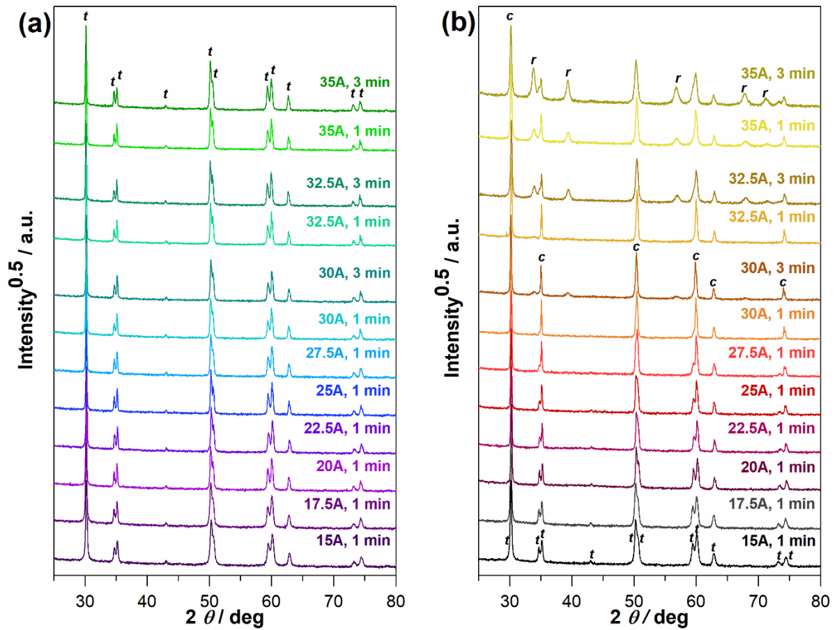
Figure 3. XRD patterns for 3YSZ samples sintered at different currents and durations under (a) Ar and (b) N 2 atmosphere. The peaks are indexed as follows: t = tetragonal zirconia, c = cubic zirconia, r = rock salt.
