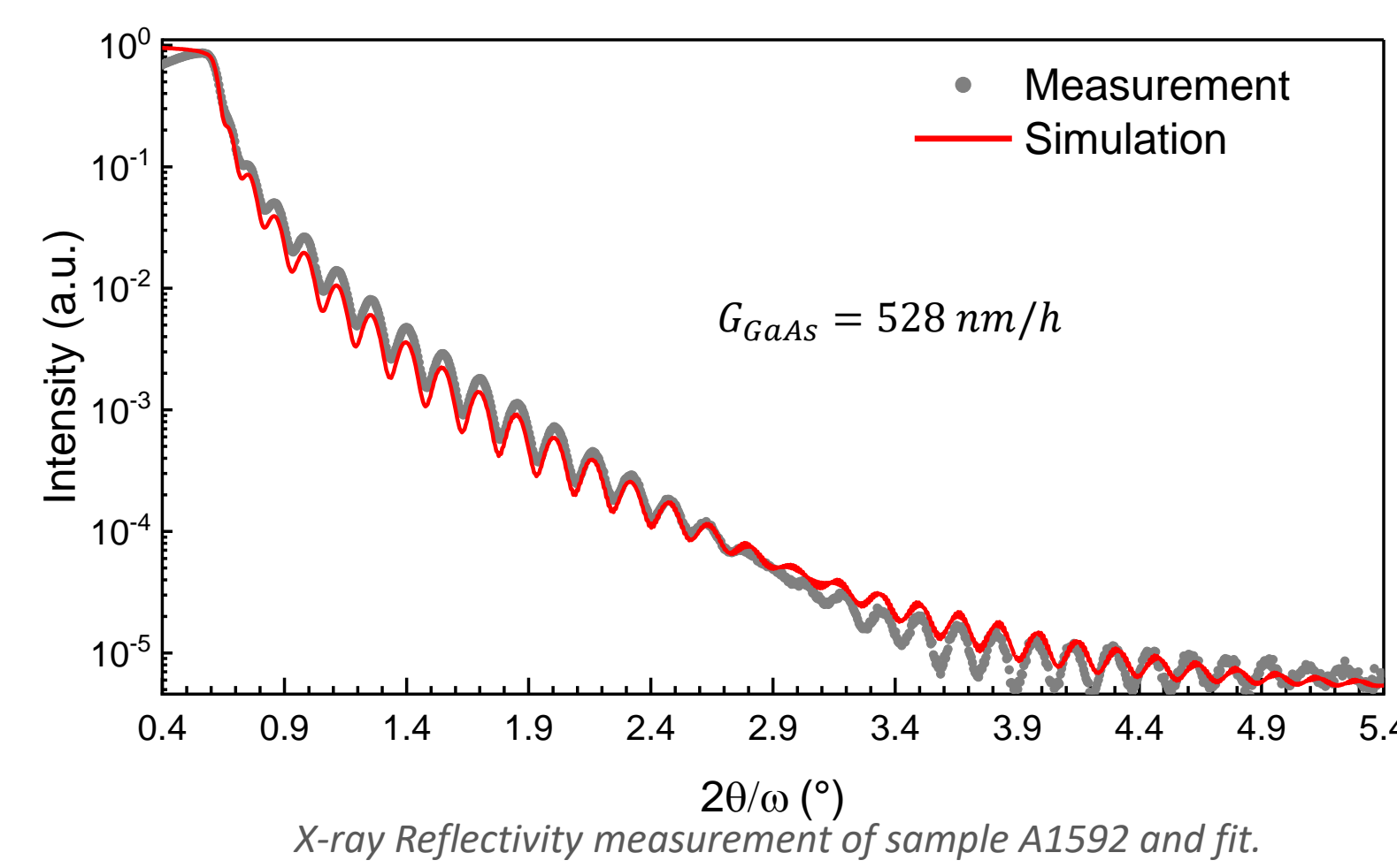
X-ray Reflectivity measurement of sample A1592 and fit.
