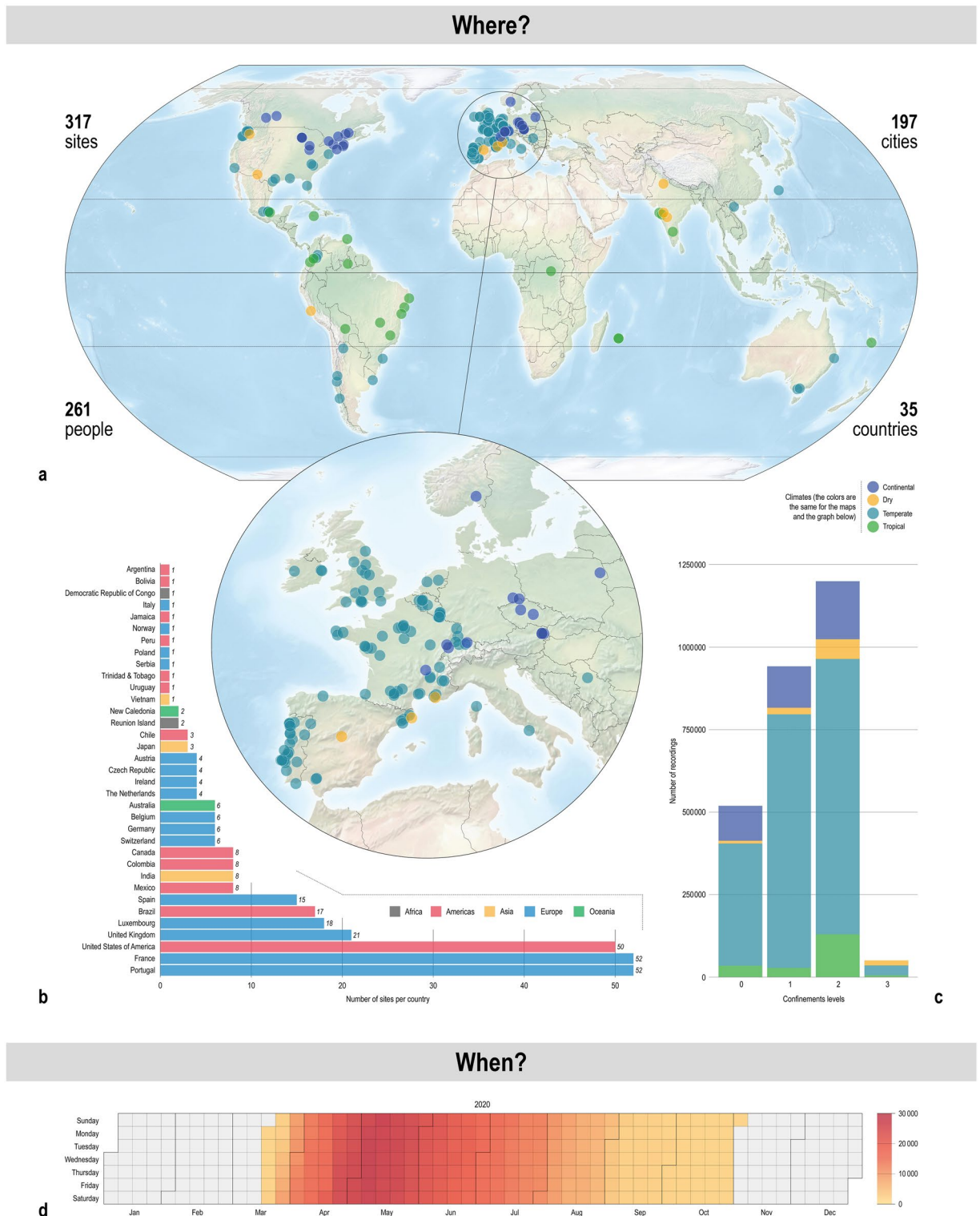
Fig. 1 Panel a. Global and European mapping of recording sites. Colors refer to climates. Panel b. Number of recording sites per country. Colors refer to continents. Panel c. Number of recordings by confinement level and climate. Panel d: temporal distribution of global sampling effort, in number of recordings.
