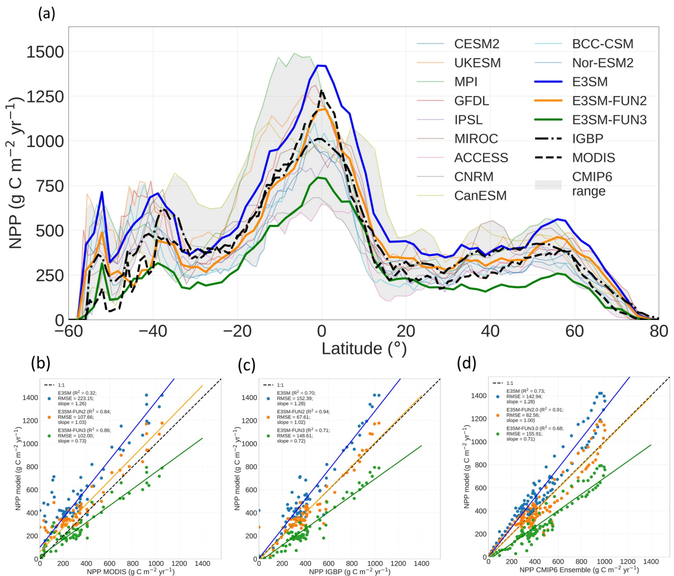
Figure 3. (a) The annual (1994–2005) zonal mean net primary production (NPP) ( \text{g C m}^{-2} \text{yr}^{-1} ) simulated by ELM, ELM-FUN2.0 (FUN2, C costs of N only), ELM-FUN3.0 (FUN3, C costs of N and P together), the zonal mean NPP from the 11-member ensemble of CMIP6 models, MODIS NPP, and IGBP NPP; (b) scatter plot between zonal mean annual NPP from three configurations of ELM (default, FUN2, and FUN3) and MODIS NPP, IGBP NPP, and NPP from the ensemble member of 11 CMIP6 models. The r^2 , RMSE, and slope values are shown in brackets.
