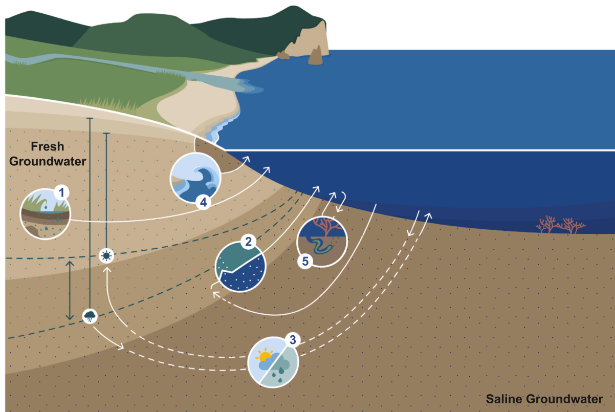
Fig. 3. Conceptual diagram of an unconfined coastal aquifer including the major Submarine Groundwater Discharge pathways, subdivided according to the driving mechanism: 1) Terrestrial groundwater discharge (usually fresh groundwater); 2) Density-driven seawater circulation; 3) Seasonal exchange of seawater; 4) Shoreface seawater circulation; and 5) cm-scale porewater exchange (PEX). Pathways 1, 2 and 3 could be extended farther offshore in systems with confined units.
