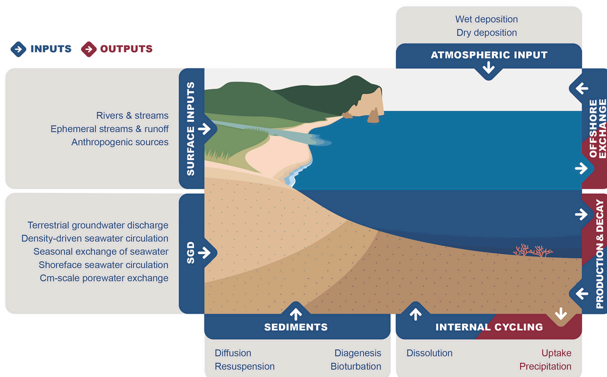
Fig. 7. Conceptual model illustrating the sources (blue) and sinks (red) of Ra isotopes in the coastal ocean. (For interpretation of the references to colour in this figure legend, the reader is referred to the web version of this article.)
