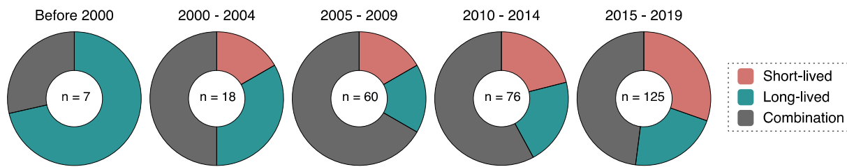
Fig. 2. Number of research articles published in 5-year periods in which Ra isotopes have been used as tracers of SGD. The articles were classified according to the Ra isotopes used: only short-lived ( ^{223}\text{Ra} and/or ^{224}\text{Ra} ), only long-lived ( ^{226}\text{Ra} and/or ^{228}\text{Ra} ) or a combination of both. The search was performed using the words “SGD or Submarine Groundwater Discharge” AND “Ra or Radium” as keywords in “Web of Science” ( n = 477 ). Reviews, method articles and studies not applying Ra isotopes as tracer of SGD-related processes were excluded from this classification. A total of 286 articles were considered in this classification analysis.
