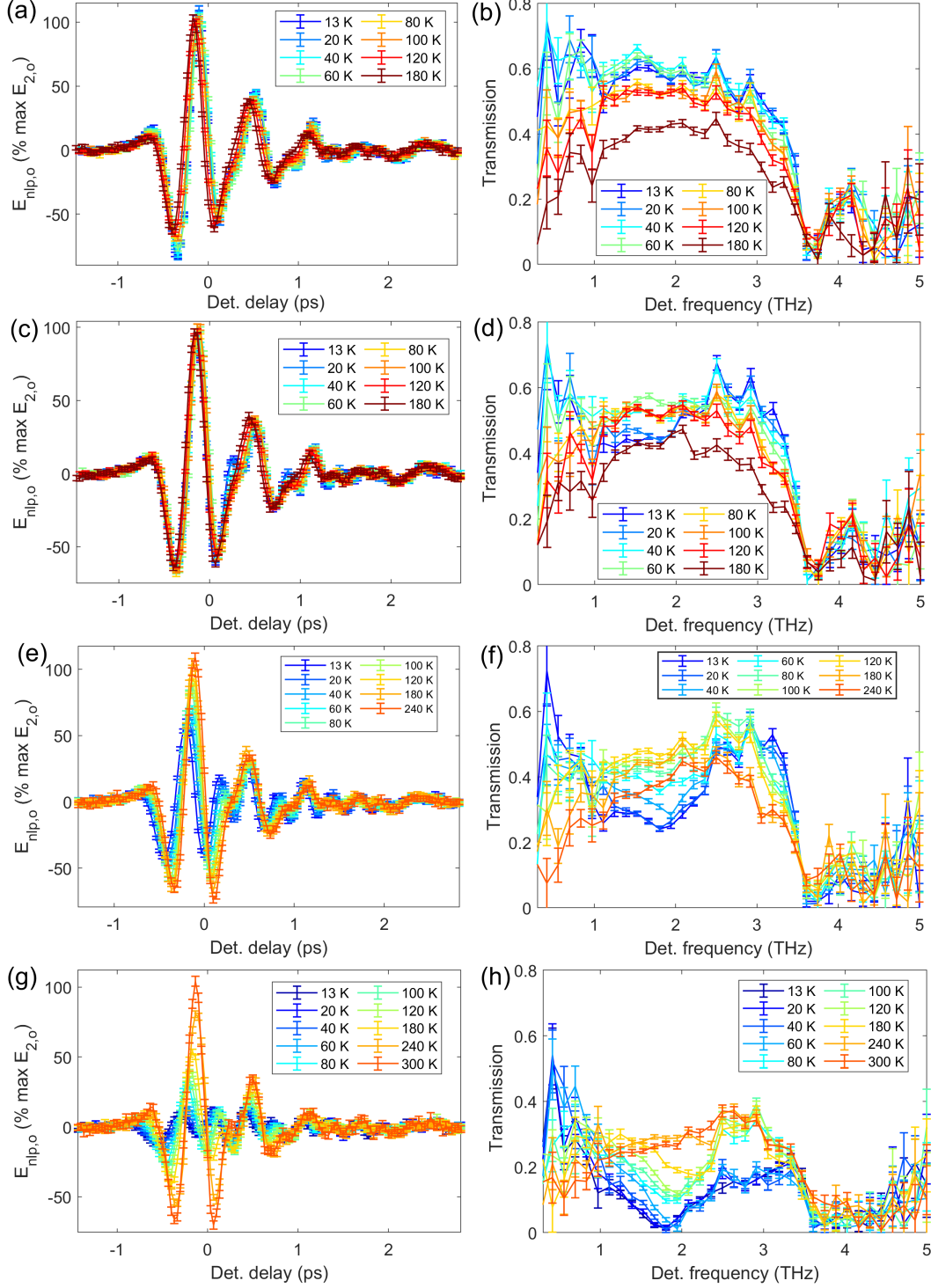
FIG. S9. Samples of typical data showing experimental uncertainties. Panels (a),(c),(e),(g) show the nonlinear probe E_{\text{nlp,o}} acquired at t_{\text{ex}} = 2.54 ps (averaged around a \pm 67 fs range) using peak fields E_{1,i} = 169.4, 50.8, 25.4, 8.5 kV/cm and E_{2,i} = 7.7 kV/cm respectively. Panels (b),(d),(f),(h) show the transmission of E_{2,i} (peak amplitude at 7.7 kV/cm) associated to the data in the corresponding panel on their left.
