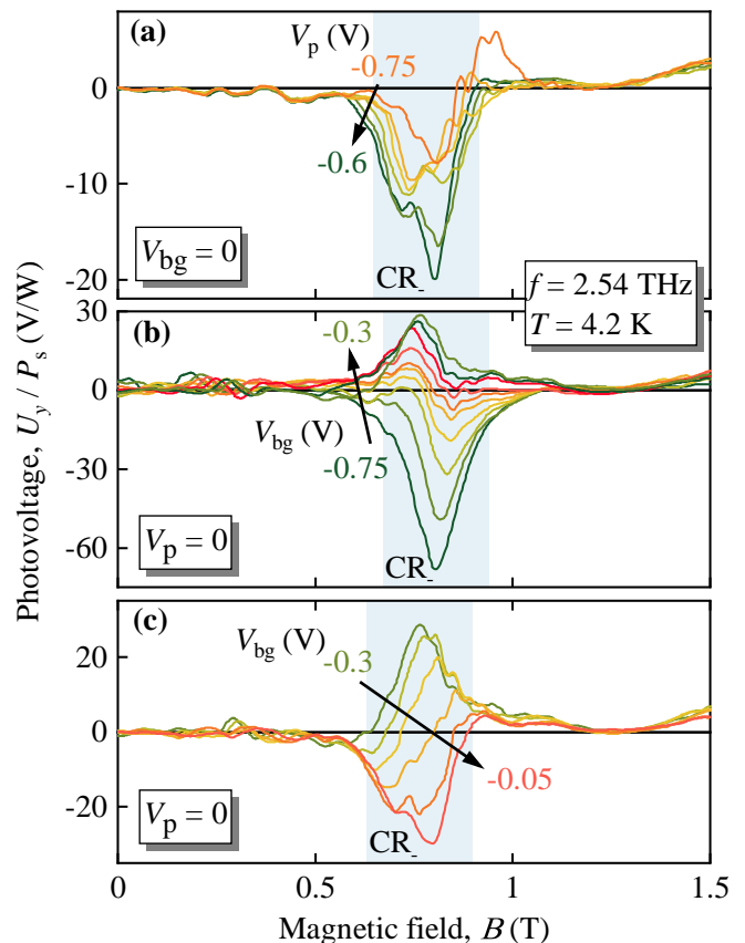
Figure 6. Figure with identical data as presented in Fig. 4 but illustrated without a vertical offset. Panel (a) corresponds to the data in Fig. 4 (b), where V_p is varied V_{bg} is fixed, whereas panel (b) and (c) show the data from Fig. 4 (c) with different V_{bg} and fixed V_p . The normalized photosignal was measured along the y -direction as a function of magnetic field for left-handed circularly polarized THz radiation ( \sigma^- ). The position of CR is highlighted by the blue shaded area and indicated with CR-.
