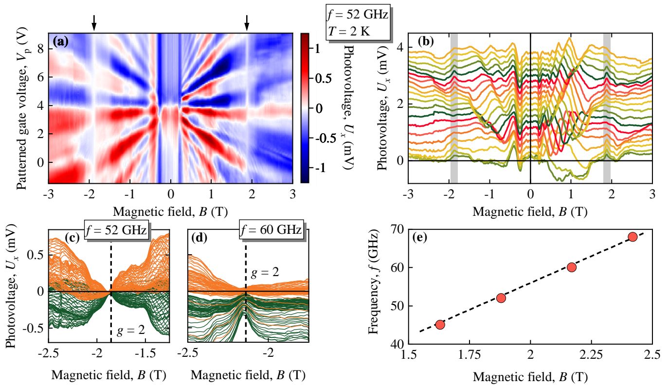
Figure 5. Magnetic field dependencies of the photocurrent excited by the microwave radiation along the Hall bar. The data are obtained for zero back gate voltage and the azimuth angle \alpha = 90^\circ . Panels (a)–(c) show the photovoltage in response to the radiation with f = 52 GHz and different patterned gate voltages. The photovoltage amplitudes in the panel (a) are indicated by the color bar on the right. The traces in the panel (b) show the magneto-ratchet signal for patterned gate voltages varied from V_p = 0.03 to 0.6 V with a step of 0.03 V. The traces are shifted vertically by 0.2 mV for clarity. Vertical arrows in the color map, panel (a), and gray shaded regions in panel (b) indicate the position of the ESR that results in a vanishing photovoltage. Panels (c) and (d) show a zoom of the data obtained for f = 52 and 60 GHz. The traces were recorded for different patterned gate voltages varying from V_p = -0.6 to 0.6 V with a step of 0.01 V. The positive (negative) V_p are shown in orange (green) color. They are shown without a vertical shift. The vertical dashed lines show the positions of the ESR for the Landé factor g = 2 . Panel (e) shows the evolution of the magnetic field position of the ESR with the excitation frequency. The dashed line is a calculated line for g = 2 . All data were recorded in sample #A.
