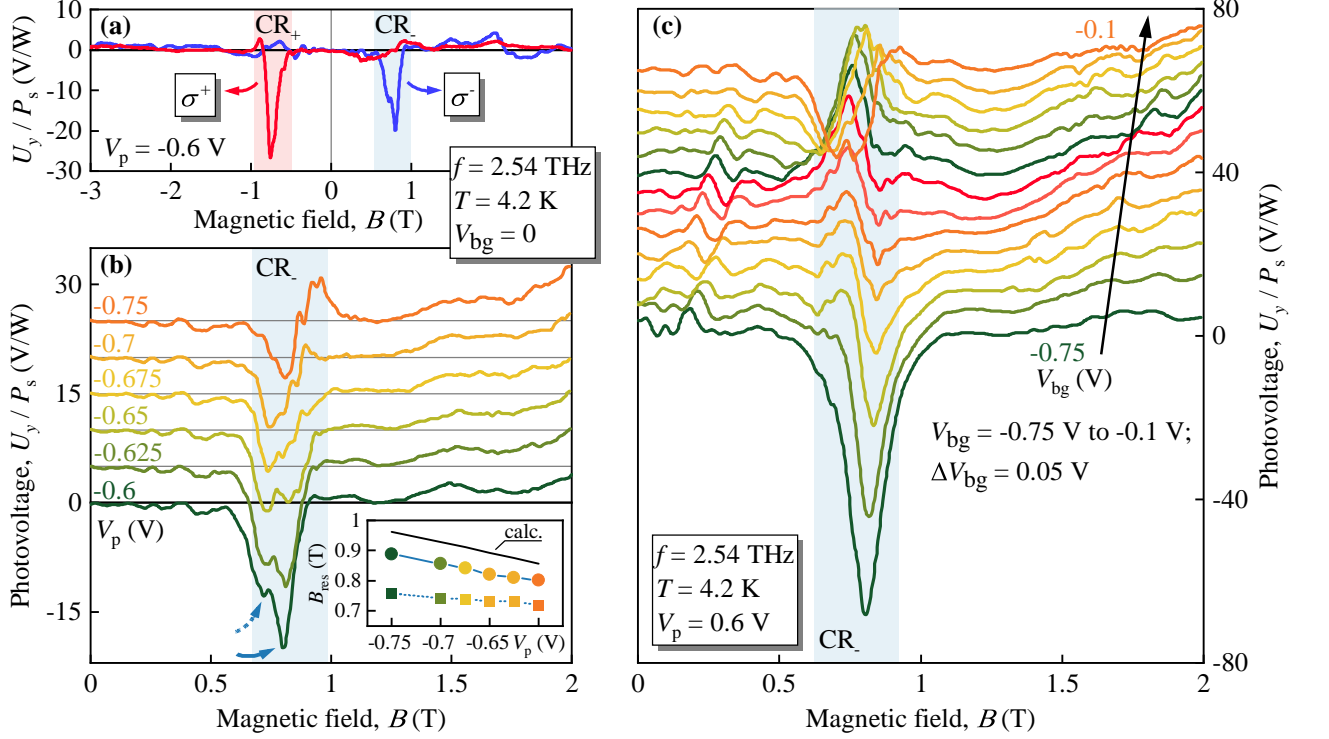
Figure 4. Normalized photosignal U_y/P_s measured along the y -direction as a function of magnetic field for the azimuth angle \alpha = 0 with f = 2.54 THz. Panel (a): Photosignal traces obtained for right-handed ( \sigma^+ , red curve) and left-handed ( \sigma^- , blue curve) circularly polarized radiation with V_{bg} = 0 . The emerging CR is highlighted by a correspondingly colored area and is named as CR + (CR - ) for \sigma^+ ( \sigma^- ). Panel (b): Photosignal traces obtained for left-handed circularly polarized radiation, V_{bg} = 0 and different patterned gate voltages. The solid and dashed blue arrow indicate the two observed resonances. The inset shows the magnetic field positions B_{res} of the resonances (colored circles) as a function of V_p . The dashed (solid) blue arrow in the main panel corresponds to the circles connected by a dashed (solid) blue line. The black solid line was calculated using the carrier densities from transport characterization. Panel (c): Photosignal traces for V_p = 0.6 V and different back gate voltages varying from -0.75 V to -0.1 V with the step of 0.05 V. The traces in panels (b) and (c) are up shifted by 5 V/W for clarity. The data were obtained in sample #A.
