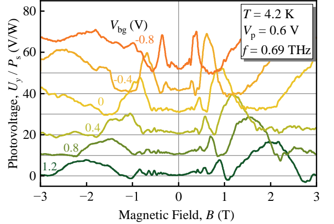
Figure B.3. Normalized photovoltage U_y/P_s measured along the basis of triangles in sample #A as a function of the magnetic field for various back gate voltages. The azimuth angle is \alpha = 90^\circ . The traces are up shifted by 10 V/W for clarity.
