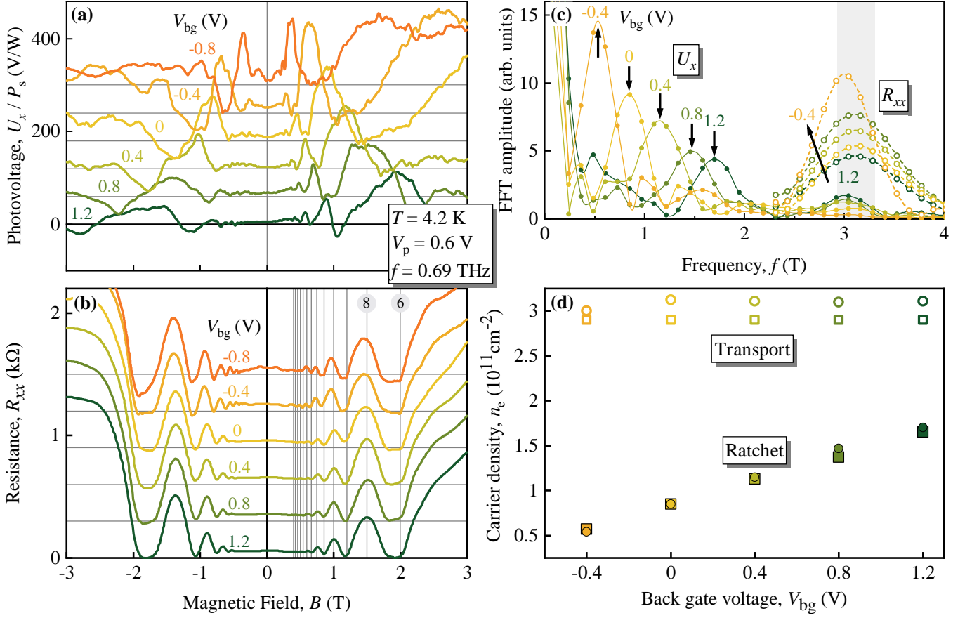
Figure 3. Panel (a): Evolution of the normalized photovoltage U_x/P_s with variation of the back gate voltage V_{bg} measured in the direction along the height of the triangles. The data were obtained for the azimuth angle \alpha = 90^\circ and a patterned gate voltage V_p = 0.6 V. The traces are shifted by 60 V/W for clarity. Panel (b): The corresponding resistance R_{xx} shifted by 0.3 k \Omega . The vertical lines indicate even filling factors of R_{xx} starting with 6 at high magnetic fields, see numbers in circles. Panel (c): the Fast Fourier transformation (FFT) analysis of the photosignal U_x (full circles and solid lines) and the longitudinal resistance R_{xx} (open circles and dashed lines) obtained for different back gate voltages indicated by numbers close to the curves. The spline lines are a guide for the eye. Panel (d): Back gate voltage dependence of the carrier density n_e obtained from the oscillations of the photosignal (full symbols) and R_{xx} (open symbols). Circles show the densities obtained from the FFT, and rectangles show the densities obtained from the filling factor analysis. The data were obtained in sample #A.
