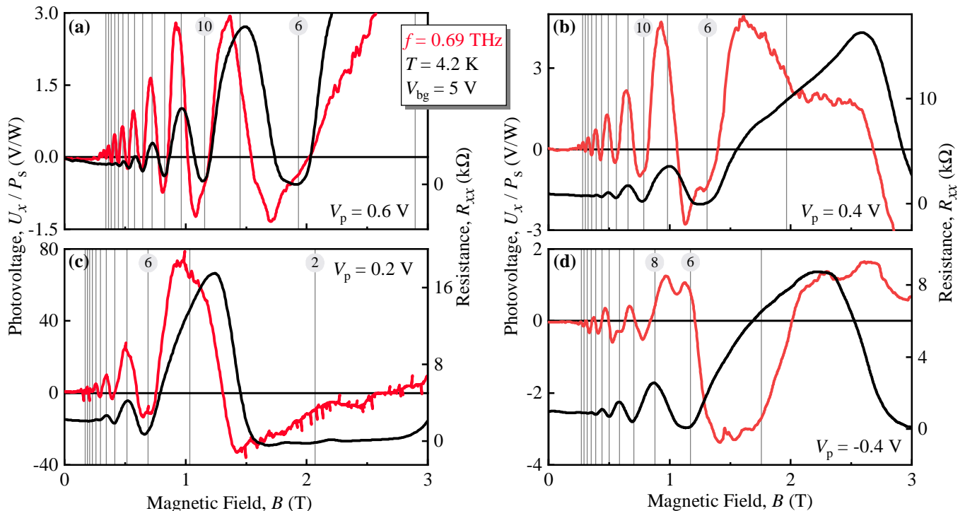
Figure 2. Photovoltage measured as a function of magnetic field in x -direction (along the triangles' height), normalized to radiation power, for different patterned gate voltages V_p at a fixed gate voltage V_{bg} . The data are obtained in sample #A for frequency 0.69 THz and radiation electric field vector parallel to x -direction ( \alpha = 90^\circ ). The corresponding resistance R_{xx} is represented by the black traces on the right axes. The vertical lines indicate even filling factors of R_{xx} counted from higher to lower magnetic fields, see numbers in circles.
