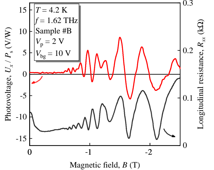
Figure C.1. Photovoltage U_x (red curve) measured along the height of triangles in sample #B as a function of the magnetic field for the azimuth angle \alpha = 90^\circ . The black curve is the corresponding resistance.
