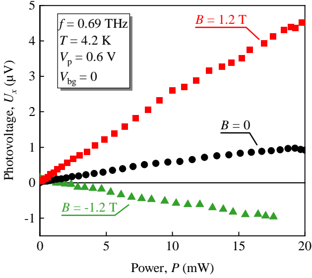
Figure B.1. Power dependence of the photovoltage measured in the x -direction in sample #A for three different values of the magnetic field, B = \{0, \pm 1.2\} T.
