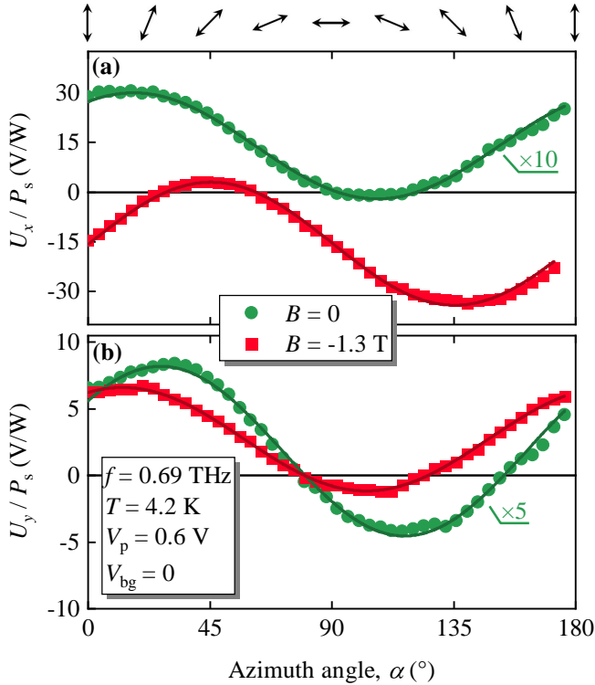
Figure B.2. Polarization dependence of the normalized photo-signal of U_x (a) and U_y (b) obtained in sample #A at B = 0 T (green traces) and B = -1.3 T (red traces).
