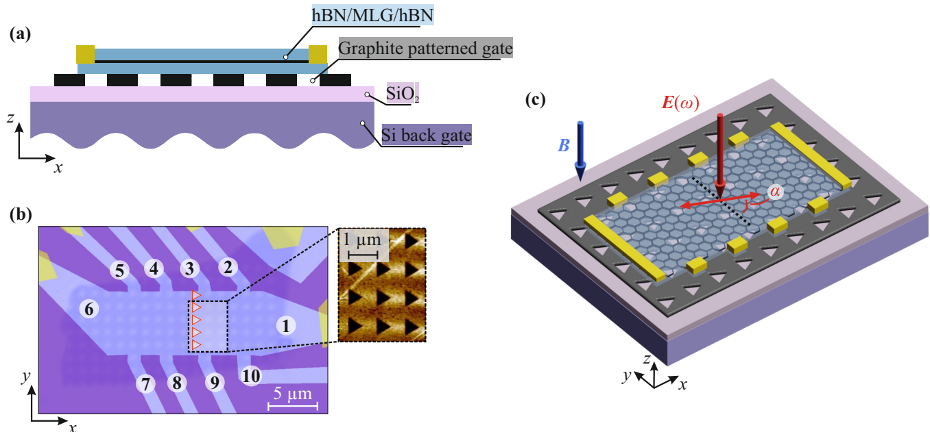
Figure 1. Sketch of the sample and the experimental setup. Panel (a): The cross section of the sample. Panel (b): Photograph of sample #A (left) and an AFM image of the periodically patterned gate (right). The patterned gate made of five graphene layers has equilateral triangular holes arranged in a square lattice. In the photo, a row of triangles is highlighted by red color. The x -direction is along the height of the triangles, and the y -direction is along their base. Panel (c): Experimental configuration. The red vertical arrow shows the normal incident linearly polarized radiation with a wavelength much larger than the lattice period d and a laser spot much larger than the Hall bar. The red double arrow sketches the radiation electric field vector \mathbf{E}(\omega) , whose orientation with respect to the triangle height is defined by the azimuth angle \alpha . The blue arrow indicates the magnetic field \mathbf{B} applied perpendicularly to the sample plane.
