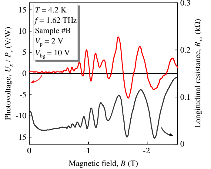
Figure C.1. Photovoltage U_x (red curve) measured along the height of triangles in sample #B as a function of the magnetic field for the azimuth angle \alpha = 90^\circ . The black curve is the corresponding resistance.
