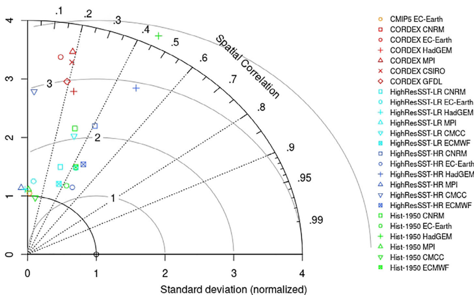
FIGURE 6 Taylor diagram of the total precipitation of the rainy season. The x-axis (y-axis) shows the normalized SD of the total precipitation of the rainy season. The curve axis shows the spatial correlation [Colour figure can be viewed at wileyonlinelibrary.com]
