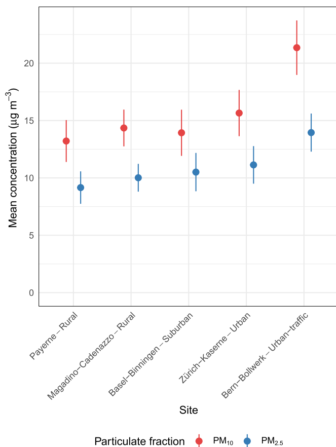
Fig. 2. Mean PM 10 and PM 2.5 concentrations for the filter-based every fourth-day sampling regime for five Swiss monitoring sites between June 2018 and May 2019.
