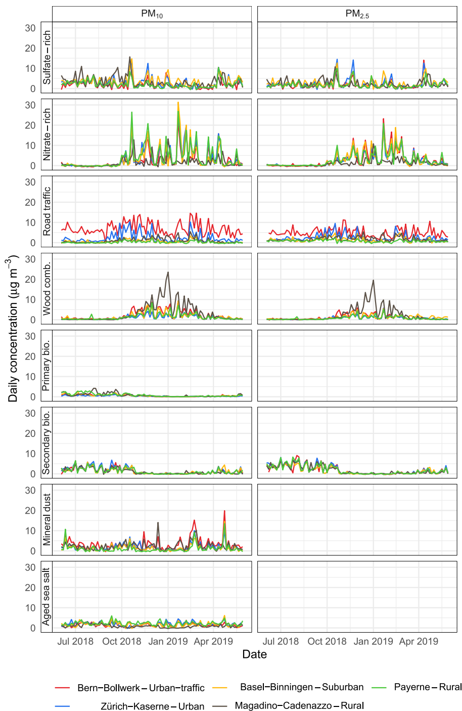
Fig. 3. Time series of the eight PMF-identified sources for PM 10 and PM 2.5 at five sampling sites in Switzerland between June 2018 and May 2019. Three of the eight sources were not identified for PM 2.5 and therefore, are not present.
