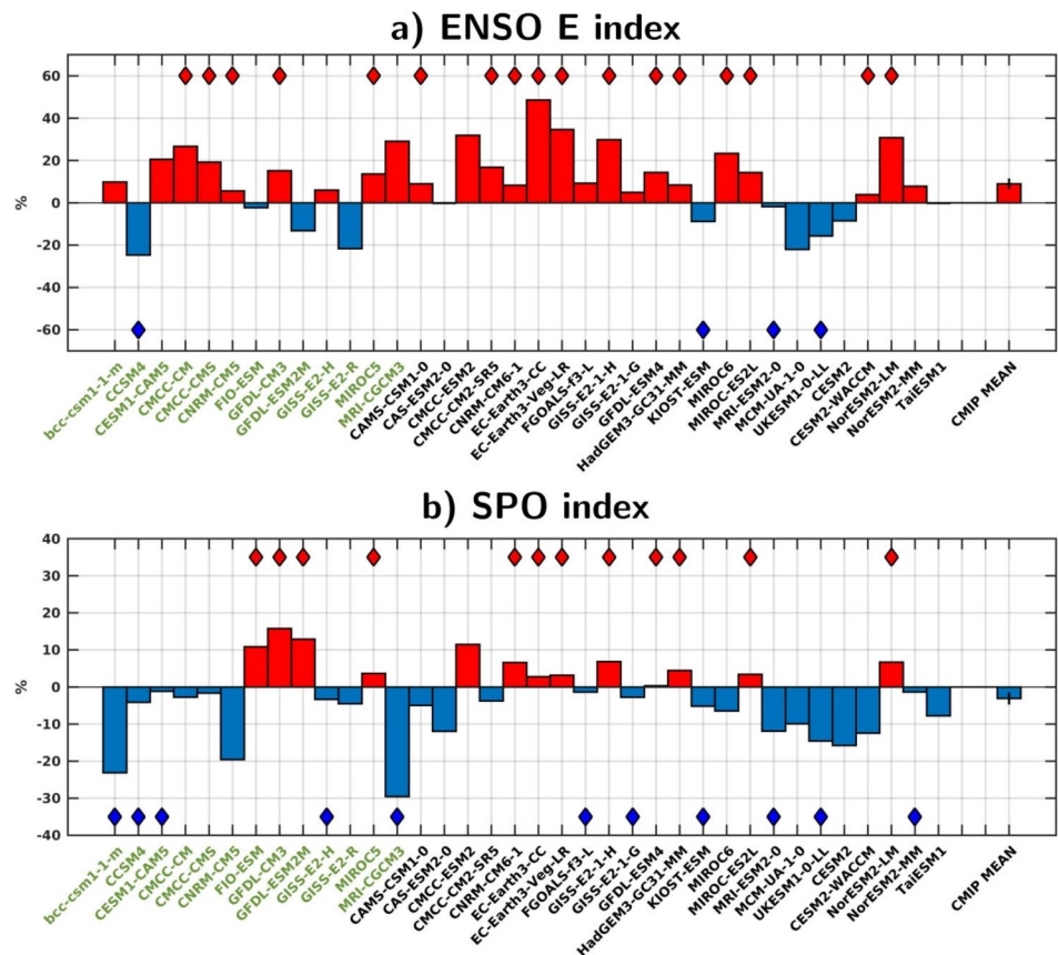
Fig. 10 Change in variability of the a E index and b SPO index between the present (1920–2014) and future (2015–2100) climate for the 36 selected models. Green (black) font in the x-axis corresponds to CMIP5 (CMIP6) models. Multi-model mean is shown with its corresponding confidence interval as a vertical segment. The confidence interval is obtained using a bootstrap method following the methodology of Cai et al. (2018), as in Fig. 5. Red (blue) diamonds indicate models for which the sign of change in CNI and E/SPO is positive (negative) for both indices
