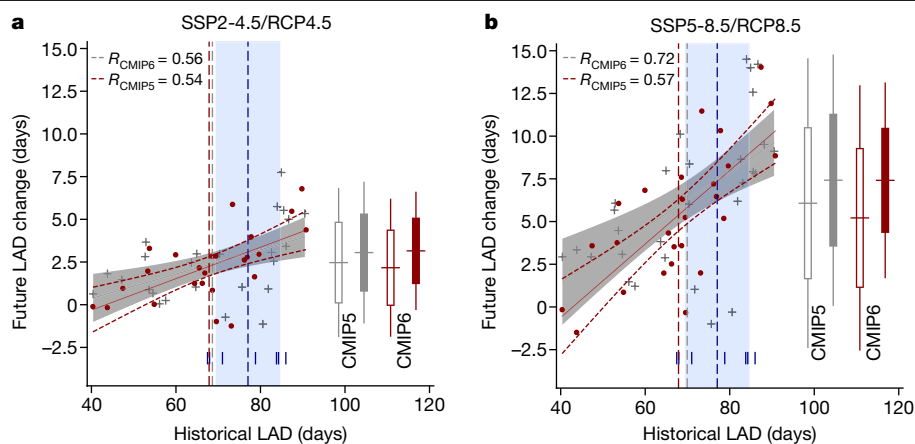
Fig. 2 | Emergent constraint on future LAD change. a, b , Inter-model relationship between historical LAD climatological mean and projected twenty-first-century LAD change from CMIP6 (red) and CMIP5 (grey) models under SSP2-4.5/RCP4.5 (a) and SSP5-8.5/RCP8.5 (b) scenarios. Every cross (CMIP5) and dot (CMIP6) represents the global (50° S–50° N) land average of a model. The corresponding MEMs are shown as vertical dashed lines.
