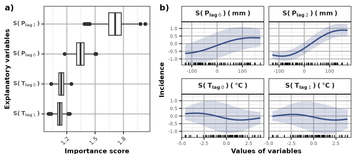
Fig 4. Effect of the explanatory variable in the SVR seasonal model. The importance score (a) represents the increase in MAE caused by repeated permutations of the variable in the dataset. The partial dependence curves (b) estimate the marginal effect of each variable by computing the average (blue line) ( \pm standard error, blue ribbon) of Individuals Conditional Expectancy (ICE) curves (see methods).
