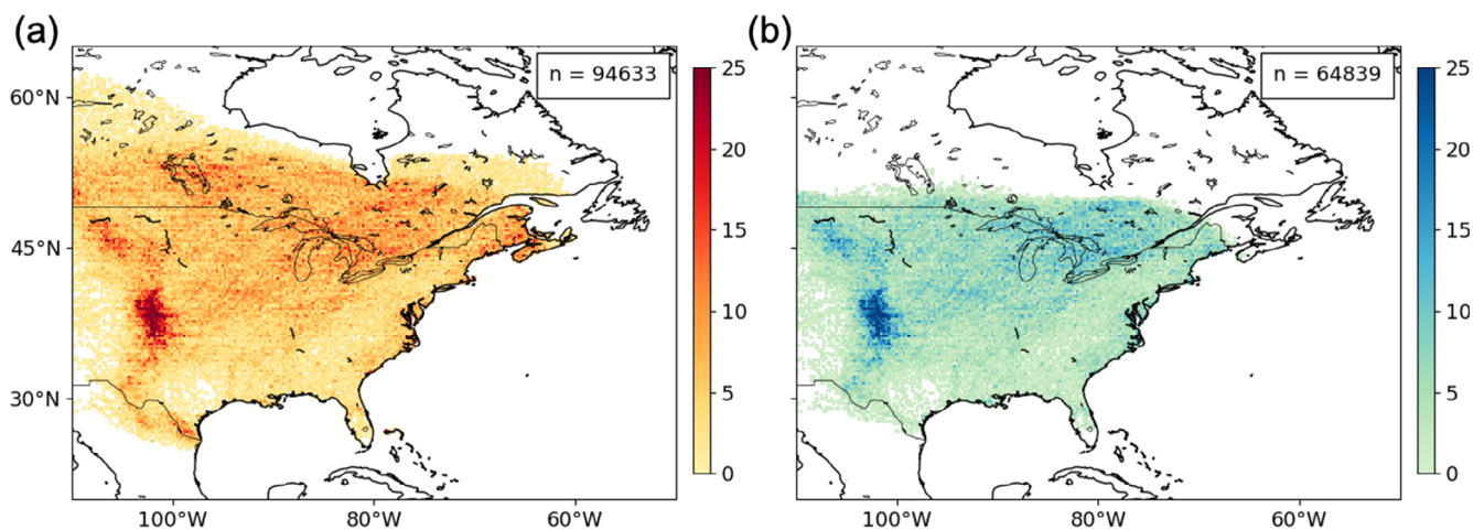
FIGURE 3 (a) Number of cyclone centres at each grid point with more than 100 10-m-wind-speed observations available within their 1000-km radius during 2005–2019 period. The total number of cyclone centres ( n ) is shown on the top right corner of each map. (b) Same as (a) but for precipitation observations. [Colour figure can be viewed at wileyonlinelibrary.com ]
