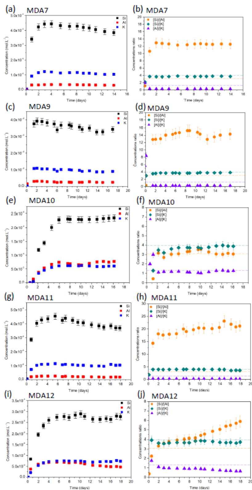
481 482 Fig. 7. Time-resolved fluid analyses of MDAc experiments. (a, c, e, g, i) Time-resolved concentrations of 483 released elements (outlet concentration subtracted from inlet concentration) and (b, d, f, h, j) ratios of these 484 concentrations. The dashed lines represent the theoretical values of the ratios calculated for stoichiometric 485 dissolution. The MDAc experiments were carried out at pH 2 and under conditions supersaturated with respect to 486 Al-bearing phases. The [Si]/[Al] and [Al]/[K] ratios reveal a lack of Al, resulting from boehmite precipitation.
