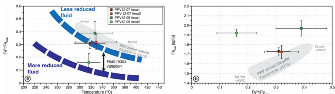
Figure 9. a XFe 3+ (Fe 3+ /Fe total ) vs temperature and b Mean values of Fe total vs XFe 3+ of chlorite particles from the damage zone in red (PPV12-07) and from the core zone in green (PPV12-05), circles for Area 1 and squares for Area 2 (cf. to Figs. 5 and 6 for analyses location). Grey diamond shapes correspond to data from Trincal et al. (2015). apfu: atoms per formula unit.
