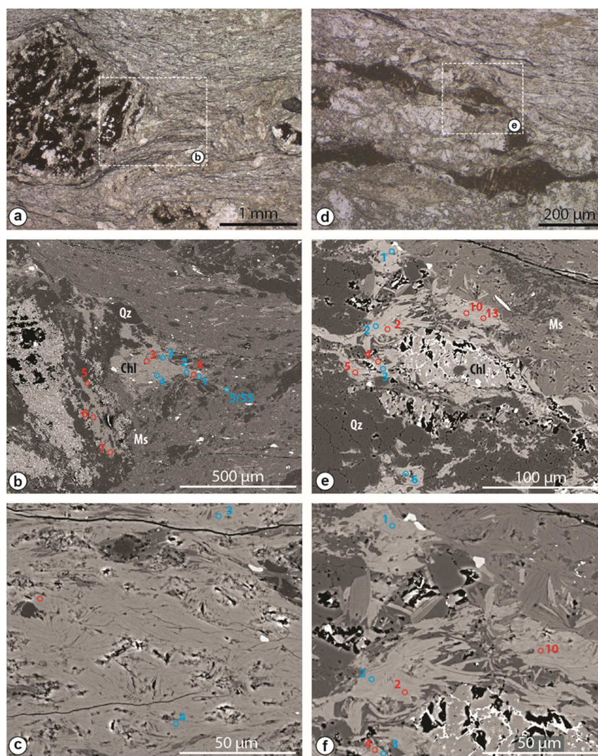
280 Figure 6. Location of analyses on PPV12-05 sample from the core zone. a to c Area 1 in Fig. 4d. a Thin-section scan image showing boudinage and schistosity-parallel quartz vein with oxide patches; Quartz + chlorite precipitated in the interboudin opening and in high angle extension veins across the early quartz vein. b SEM image showing chlorite in the strain shadow at the edge of boudinage opening (cf. frame in a). The location of the \mu -XANES analyses is in blue, and the microprobe analyses are in red. c Detail of the chlorite particles morphology. d to f Area 2 in Fig. 4d. d Optical microscope image showing an early, schistosity-parallel quartz vein deformed by shear bands with mylonitized quartz and chlorite precipitation. e SEM image Showing chlorite located at the edge of a shear vein of quartz + chlorite (cf. frame in d). The location of the \mu -XANES analyses is in blue, and the microprobe analyses are in red. f Detail of chlorite particles morphology. Elongated chlorite particles are imbricated with quartz grains. 285
