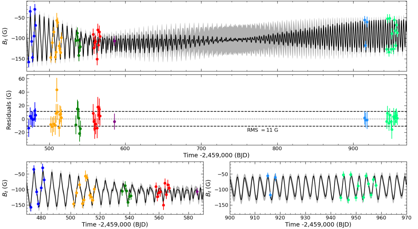
Figure 3. Gaussian process analysis of the longitudinal magnetic field of GM Aur. The top panel illustrates longitudinal magnetic field measurements (colored circles) alongside the GP-prediction values (black line). 1-\sigma error bars are depicted for both measurements and predictions. Colors represent SPIRou runs: September (blue), October (orange), November (green), and December 2021 (red), January and December 2022 (purple and light blue, respectively), and January 2023 (light green). The second panel shows residuals (observed minus modeled field). The last row offers detailed views of observations from October 2021 to January 2022 (left-hand panel) and December 2022 to January 2023 (right-hand panel).
