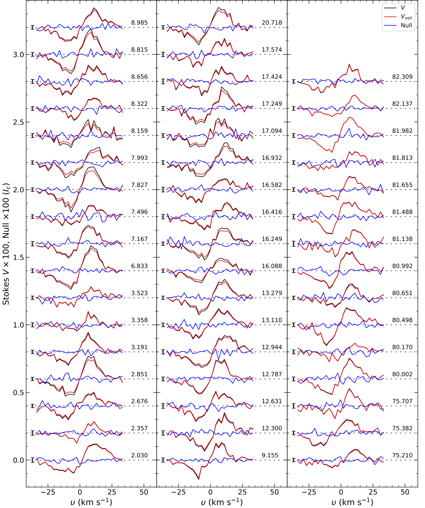
Figure B2. Unveiled (black lines, V ) and veiled (red lines, V_{\text{veil}} ) polarized LSD profiles of GM Aur. Control null polarisation profiles are shown as blue continuous lines to evidence the lack of spurious polarisation signatures in the Stokes V LSD profiles. Rotational cycles and 1-\sigma error bars (scaled following Eq. B4) are shown next to each profile.
