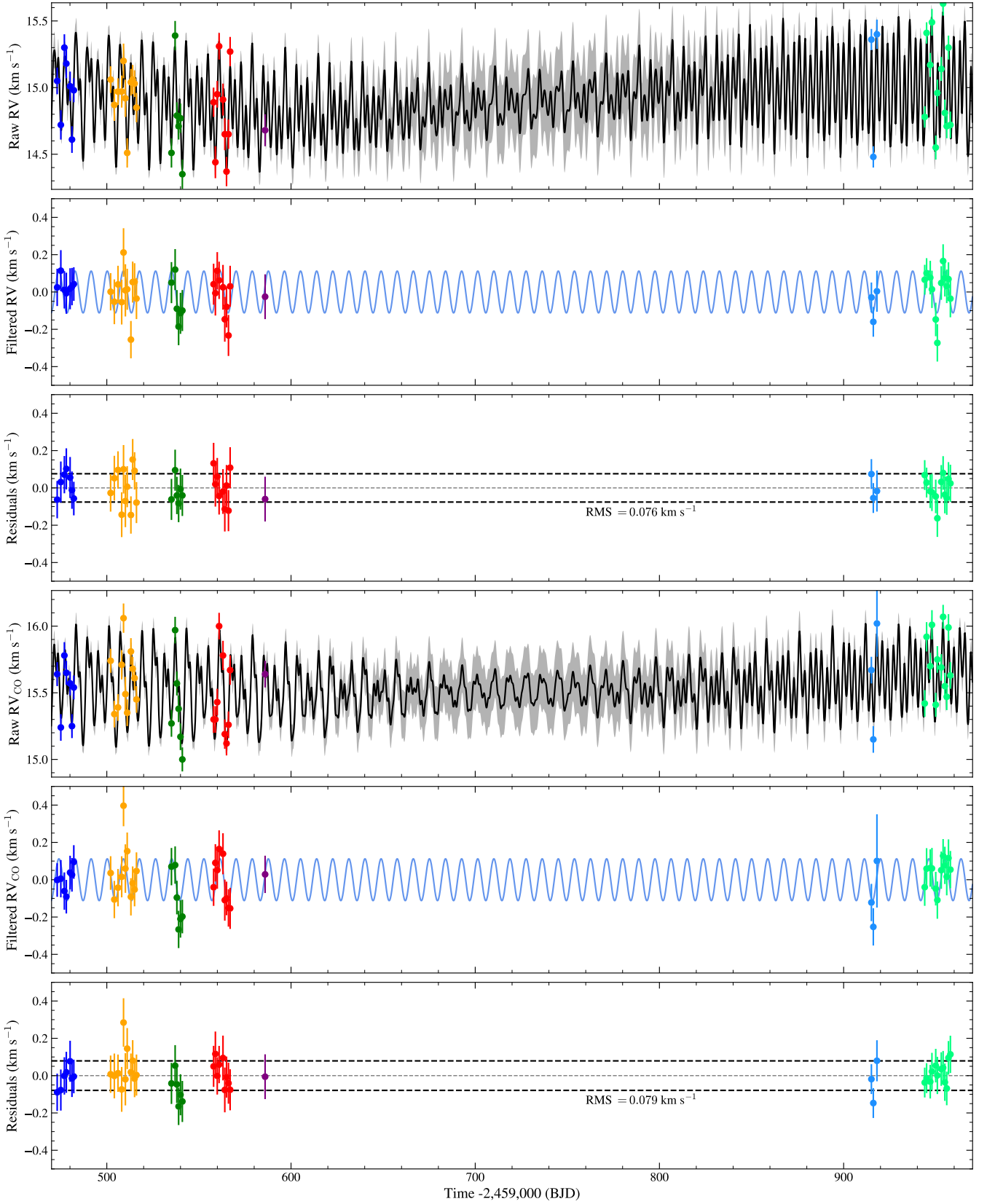
Figure 6. Joint GP regression of the raw RVs from both atomic lines (first 3 rows) and CO lines (last 3 rows) of GM Aur. Rows 1 and 4 illustrate the raw RVs alongside the GP+Planet model prediction. Rows 2 and 5 show the activity-filtered RV data and the modelled planetary RV signal (blue curve). Rows 3 and 6 give activity- and planet-filtered RV residuals. Symbol colors carry the same meaning as in Fig. 3.
