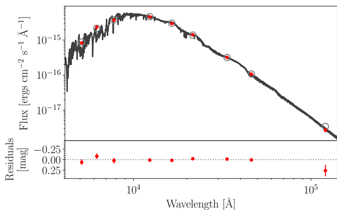
Fig. 5. SED of TOI-4860. The solid line is the MAP PHOENIX/BT-Settl-interpolated synthetic spectrum, red circles are the absolute photometric observations (the jitter has been added quadratically to the data error bars), and grey open circles are the result of integrating the synthetic spectrum into the observed bandpasses.
