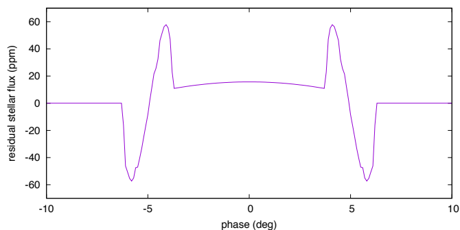
Fig. 9. Difference between the transit light curves of an ellipsoidal and a spherical planet for TOI-4860 b, obtained with uniform stellar flux.
