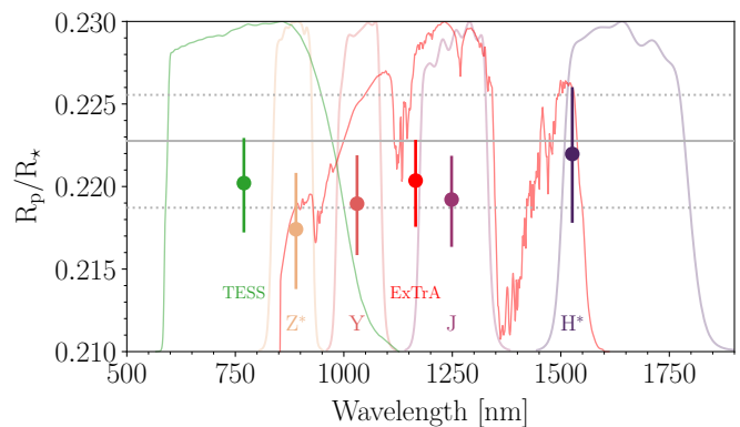
Fig. 6. Posterior distribution comparison for R_p/R_* (error bars) computed for different bands (shown and labelled with different colours). TESS, ExTrA (0.85 to 1.55 \mu\text{m} ), Z*, Y, J, and H* data are fitted jointly with a different R_p/R_* parameter for each of the datasets. The horizontal solid and dotted grey lines represent the posterior median and 68.3% CI of R_p/R_* inferred in Sect. 4.4.
