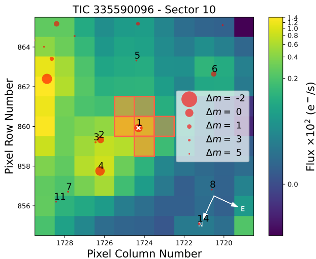
Fig. 2. TESS TPF image of TOI-4860 in Sector 10 (created with tpfplotter ; Aller et al. 2020 ). The electron counts are colour-coded. The red-bordered pixels are used in the SAP. The size of the red circles indicates the Gaia Data Release 2 magnitudes of all nearby stars ( Gaia Collaboration et al. 2018 ).
