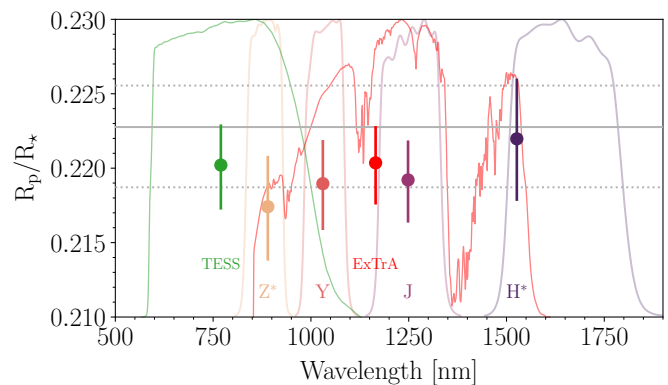
Fig. 6. Posterior distribution comparison for R_p/R_\star (error bars) computed for different bands (shown and labelled with different colours). TESS, ExTrA (0.85 to 1.55 \mu\text{m} ), Z*, Y, J, and H* data are fitted jointly with a different R_p/R_\star parameter for each of the datasets. The horizontal solid and dotted grey lines represent the posterior median and 68.3% CI of R_p/R_\star inferred in Sect. 4.4.
