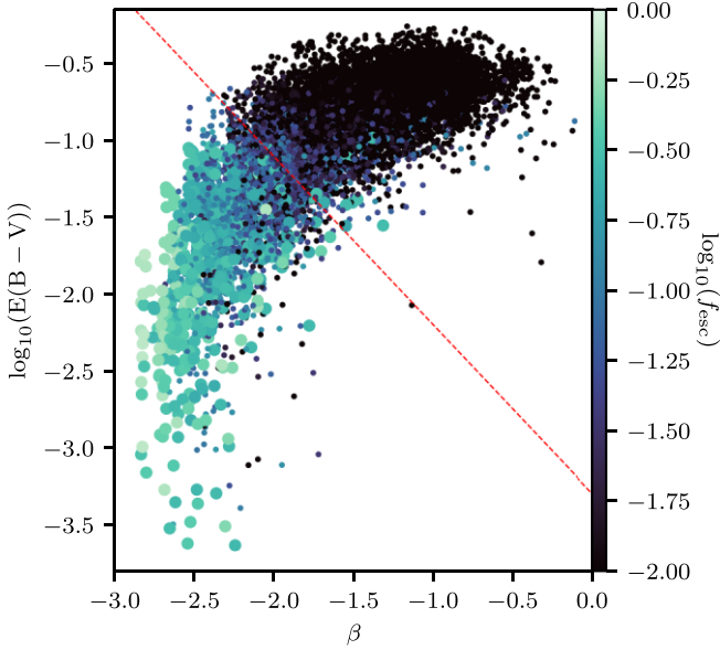
Figure 14. Line-of-sight measurements of \beta as a function of E(B - V) for all observations of galaxies in our sample with observed \log_{10}(\text{H}\alpha/L_{1500}) < 1.6 coloured by the true LyC escape fraction. Systems with escape fractions greater than 20 per cent are enlarged. A selection has been made (red, given by equation 3) to produce a sample of highly enriched leakers, 67 per cent of which have f_{\text{esc}} > 5 per cent. Those selected by this set of criteria account for 62 per cent of the total population of such systems in our sample.
