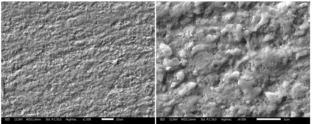
Fig. 3SI. High magnification SEM image of the surface of the 3D-printed \text{Si}_{12.6}\text{SiC}_{40.0}\text{@R120}_{14} sample.
