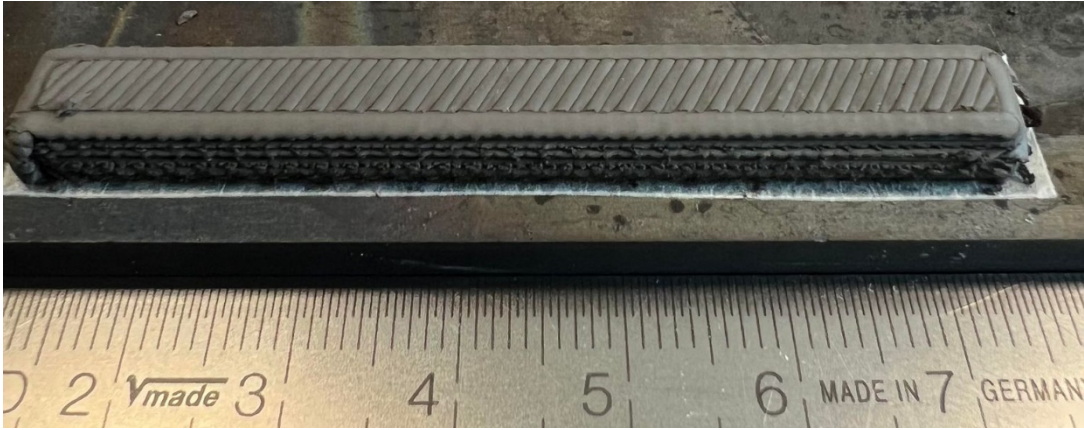
Fig. 6SI. Representative 3D printed \text{Si}_{12.6}\text{SiC}_{40.0}\text{@R120-14} sample for flexural tests.
