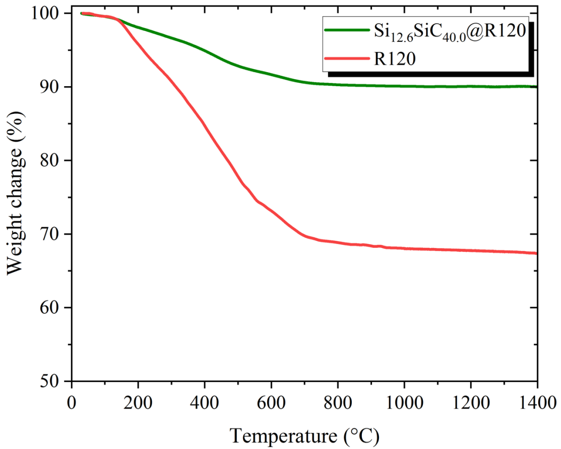
Fig. 2SI. TG investigation of the \text{Si}_{12.6}\text{SiC}_{40.0}\text{@R120} sample (compared to the R120 sample) during heat-treatment to 1400°C in flowing argon.
