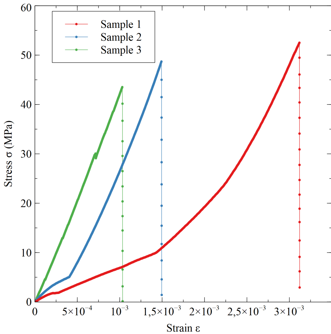
Fig. 7SI. Representative flexural stress-strain curves of 3D-printed \text{Si}_{12.6}\text{SiC}_{40.0}\text{@R120\_14} samples.
