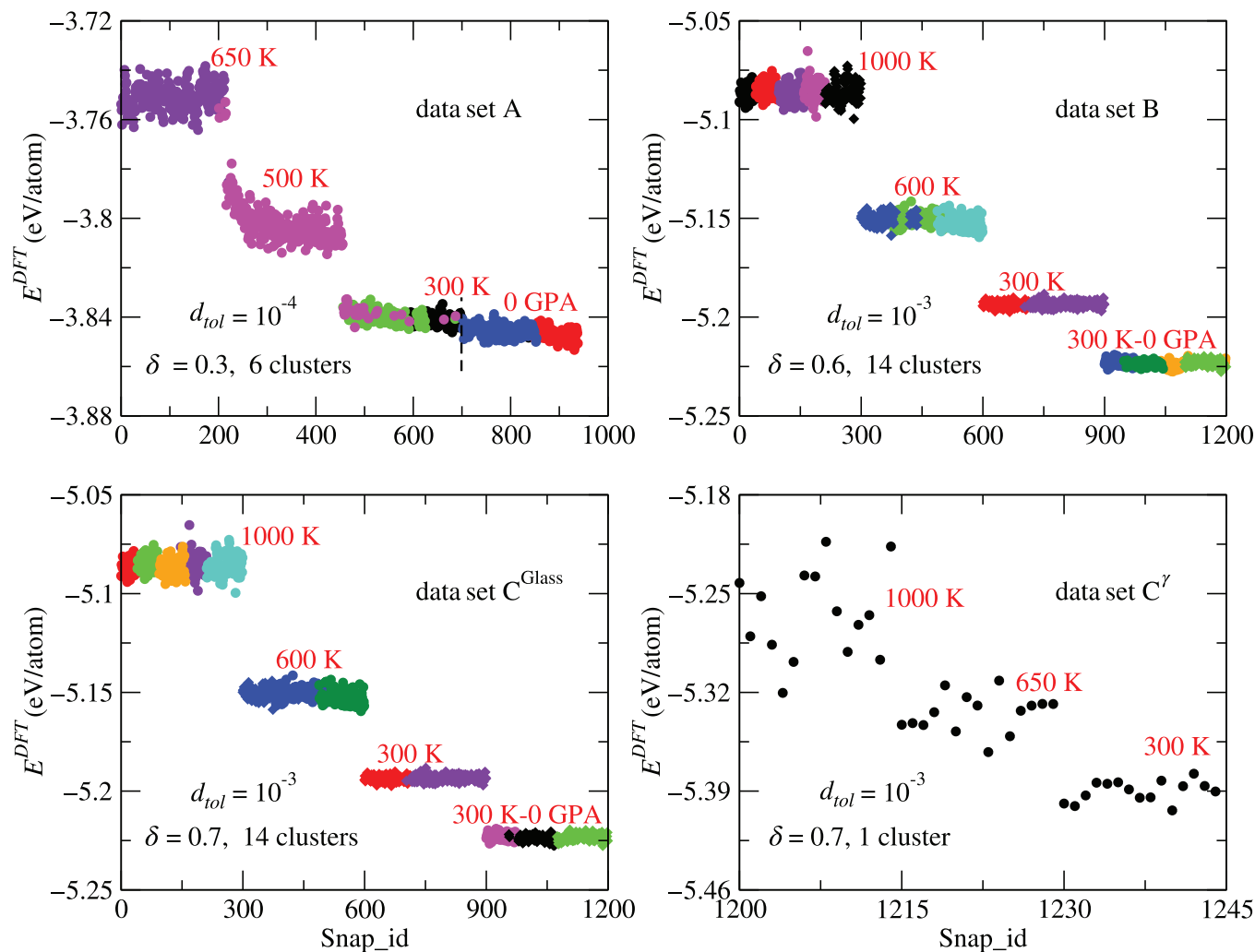
FIGURE 3 Clusters used to generate a machine learning interatomic potential (MLIP) for each of the studied systems with their corresponding value of \delta . Point distributions for data sets of 937, 1200, and 1245 points, for \text{AsTe}_3 (data set A), \text{TeO}_2^{\text{G}} (data set B), and \text{TeO}_2^{\text{G}+\gamma} (data set C), respectively. Dataset C is slit into the bottom two panels for a better visibility of the configurations of \gamma – \text{TeO}_2 . Points are colored according to the cluster to which they are assigned.
