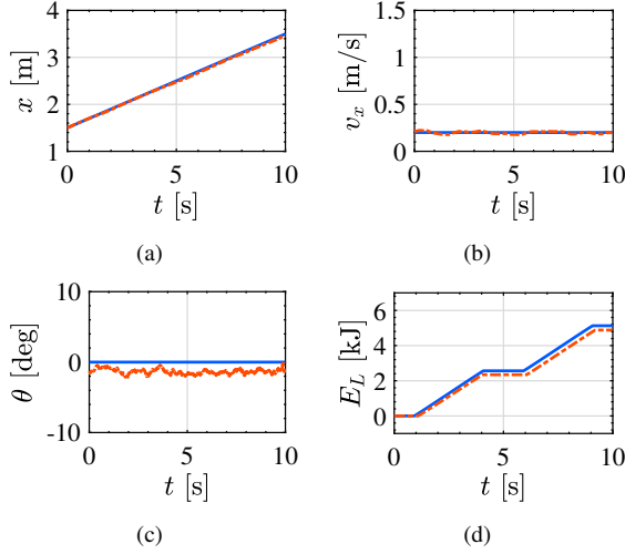
Fig. 13. Experimental results of straight trajectory. Reference value (—) and measured value (---). (a) Position x (b) Velocity v_x (c) Pitch angle \theta (d) Receiving energy E_L
