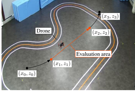
Fig. 12. Experimental setups.
