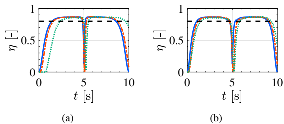
Fig. 16. Transmission efficiency in proposed trajectory. Designed value (—), simulation value (---), and experimental value (····). (a) Optimal pitch trajectory (b) Edge pitch trajectory
