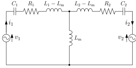
Fig. 2. Equivalent circuit of inductive power transfer system.
