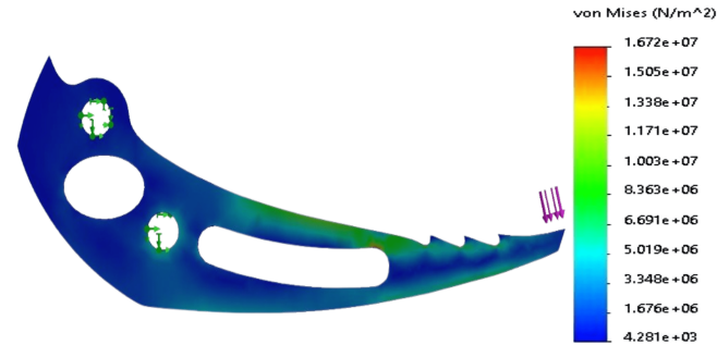
Fig. 6: Finite Element Analysis applied to the gripper's claw
