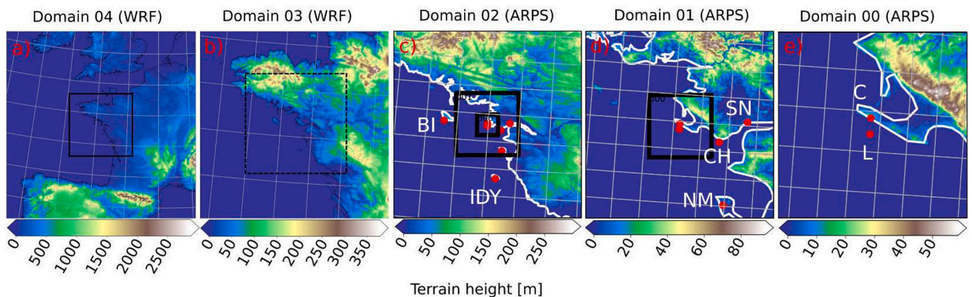
Fig. 1. Domain configuration of the WRF and ARPS nested simulations with topography. Domains d04 and d03 are WRF. Domains d02, d01 and d00 are ARPS. The red dots represent locations where simulated (ARPS) data is compared to experimental observations: L (LiDAR), C (Croisic, physical position of the LiDAR and real data probes for the aerosol), CH (Chemoulin), SN (St Nazaire), NM (Noirmoutier), IDY (Ile d'Yeu) and BI (Belle Ile). (For interpretation of the references to colour in this figure legend, the reader is referred to the web version of this article.)
