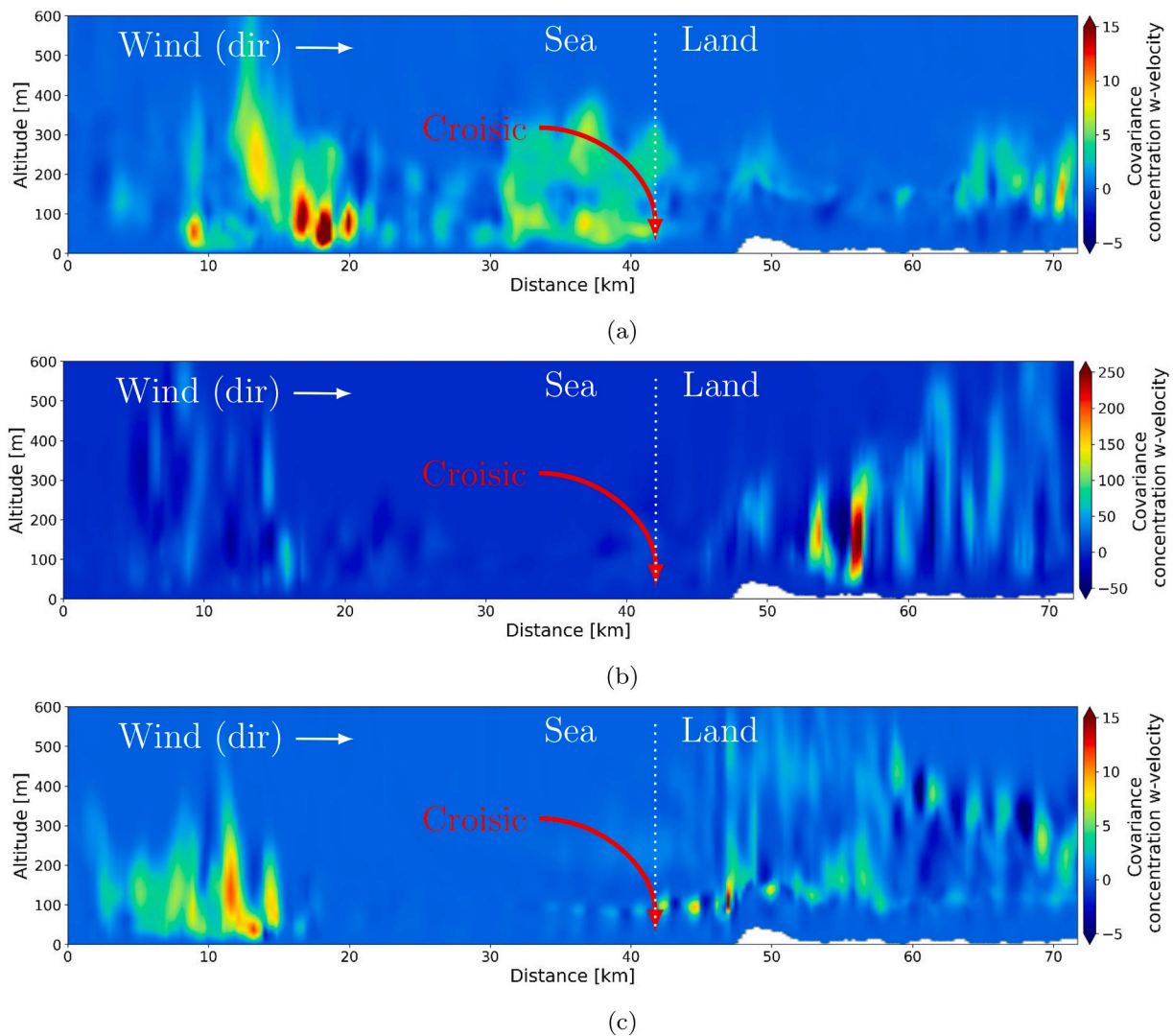
Fig. 12. Vertical turbulent flux \overline{c'w'} [ \text{m}^{-2}\cdot\text{s}^{-1}\cdot\mu\text{m}^{-1} ] of sea-spray aerosols ( r_b = 5.0 \mu\text{m} ) on domain d01 at different times on 18 June 2020: 06:00 UTC (a), 14:00 UTC (b) and 20:00 UTC (c). The same vertical cross-sections as in Fig. 9 are presented.
