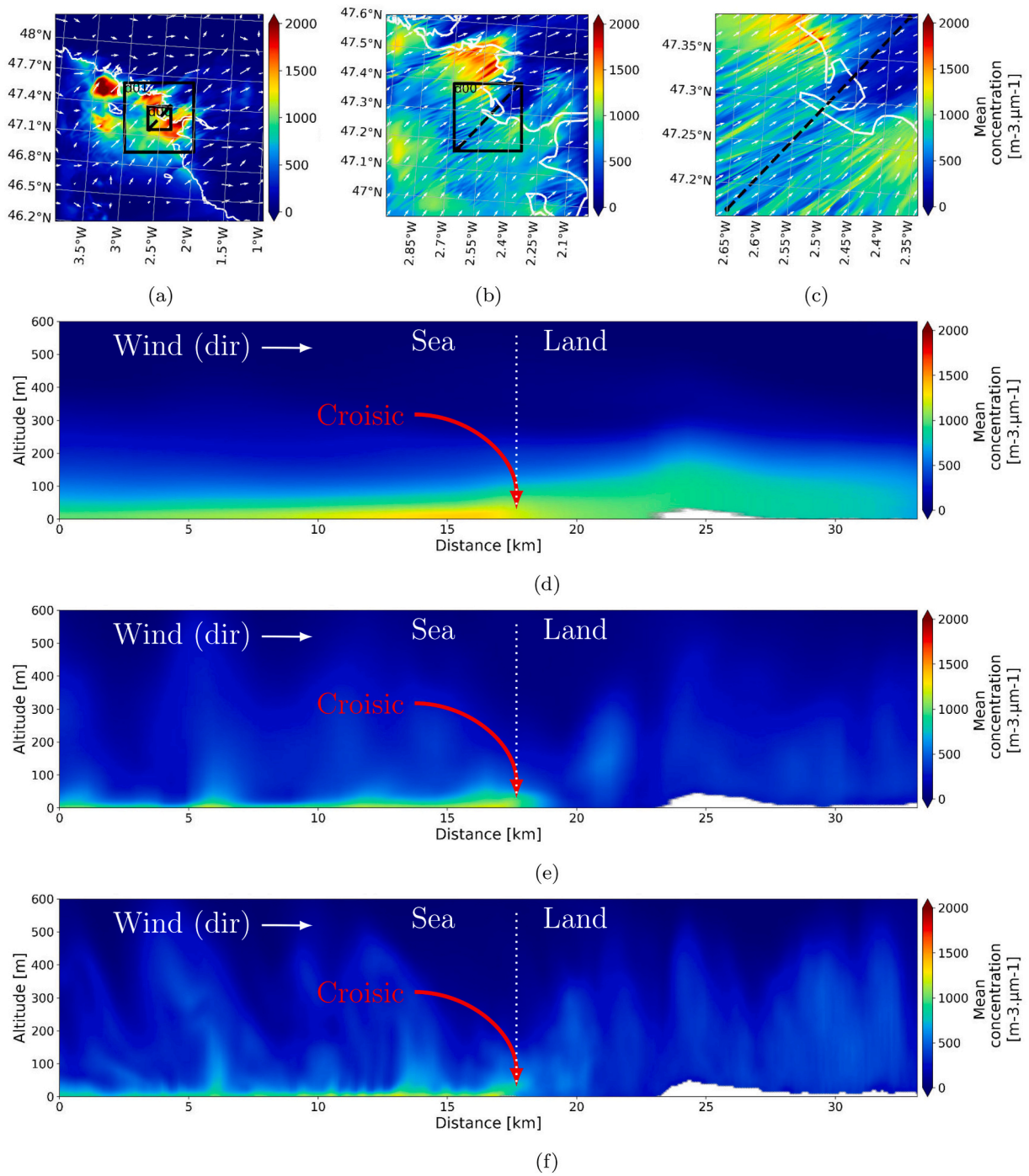
Fig. 7. Averaged sea-spray concentration [m^{-3} \cdot \mu m^{-1}] for r_b = 5 \mu m at 12:00 UTC on 18 June 2020 for domains: d02 (a, d), d01 (b, e) and d00 (c, f). Horizontal cross-sections at 20 m a.g.l. (a, b and c) and vertical cross-sections (d, e and f) indicated by the black dashed line in (a), (b) and (c), are presented. The white vectors indicate the wind velocity. The colours represent the sea-spray concentration. Topographic elements are in white in (d), (e) and (f).
