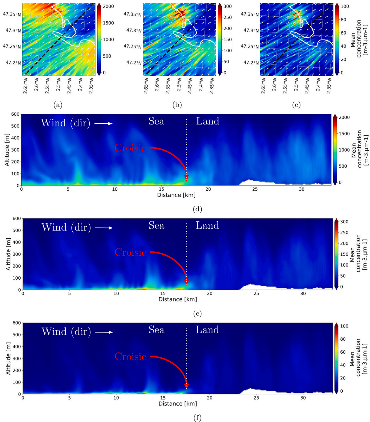
Fig. 8. Averaged sea-spray concentration [\text{m}^{-3} \cdot \mu\text{m}^{-1}] in domain d00 at 12:00 UTC on 18 June 2020 for different radii r_b : 2.5 \mu\text{m} (a and d), 10 \mu\text{m} (b and e) and 20 \mu\text{m} (c and f). Horizontal cross-sections at 20 m a.g.l. (a, b and c) and vertical cross-sections (d, e and f) indicated by the black dashed line in (a), (b) and (c), are presented. The white vectors indicate the wind velocity. The colours represent the sea-spray concentration. Topographic elements are in white in (d), (e) and (f).
