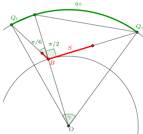
FIGURE 9. A marginal picture to the case 3.1: middle component, n = 2, m = 2 .
