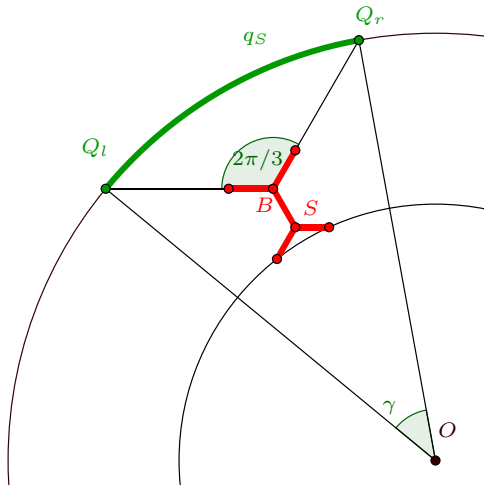
FIGURE 8. A general picture to the case 3.1: middle component, n = 2, m = 2 .
