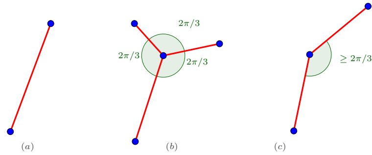
FIGURE 20. Locally minimal networks for sets of 2 and 3 points.
