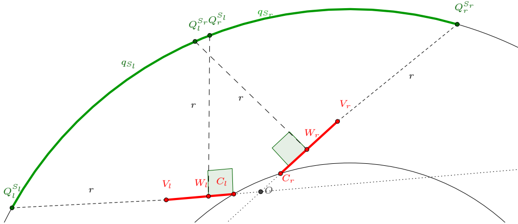
FIGURE 6. Picture to Lemma 2.18.
