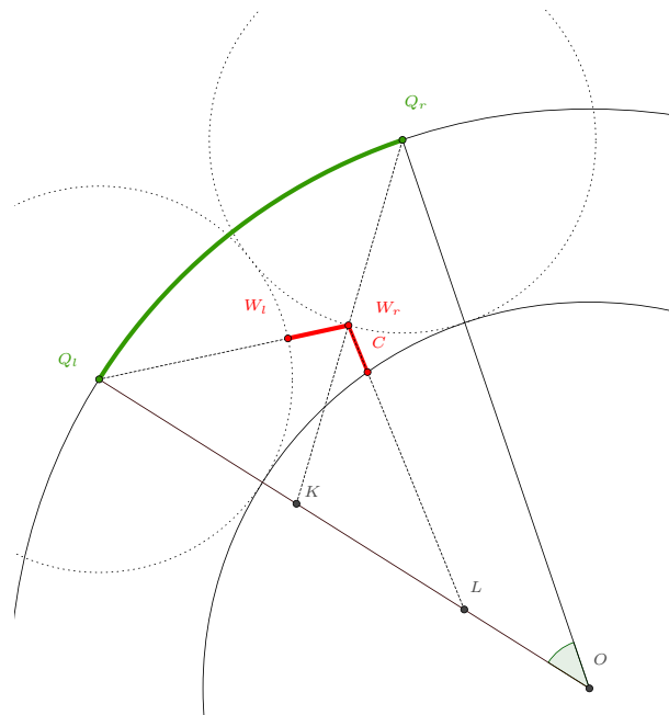
FIGURE 19. Picture to the case 3.1: ending component, n = 2, m = 1 .
