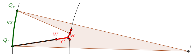
FIGURE 15. Picture to the case 3.1: middle component, m = 2, n = 1 .
