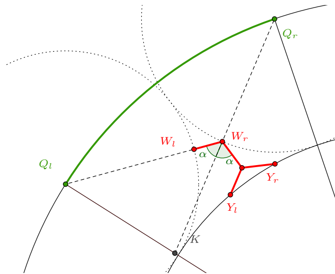
FIGURE 11. Picture to the case 3.1: middle component, n = 2, m = 2 .
