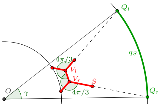
FIGURE 7. Picture to the case 3.1: middle component, n = 2, m = 2 .
