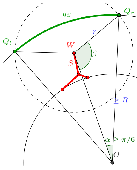
FIGURE 13. Picture to the case 3.1: middle component, m = 2, n = 1 .
