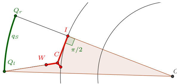
FIGURE 14. Picture to the case 3.1: middle component, m = 2, n = 1 .
