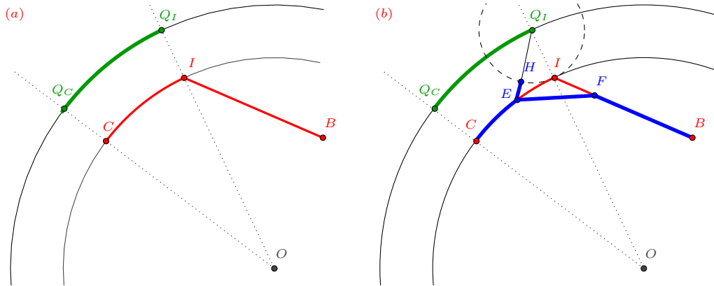
FIGURE 4. The case (iv) of Lemma 2.13: (a) the (impossible) part of the minimizer; (b) the better competitor.
