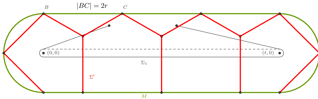
FIGURE 2. The horseshoe \Sigma_1 and the better competitor \Sigma' in Example 2.5.
