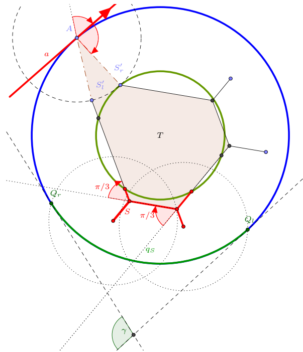
FIGURE 3. Figure to the construction of T .
