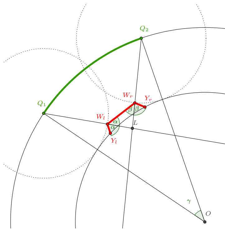
FIGURE 12. Picture to the case 3.1: middle component, n = 2, m = 2 .
