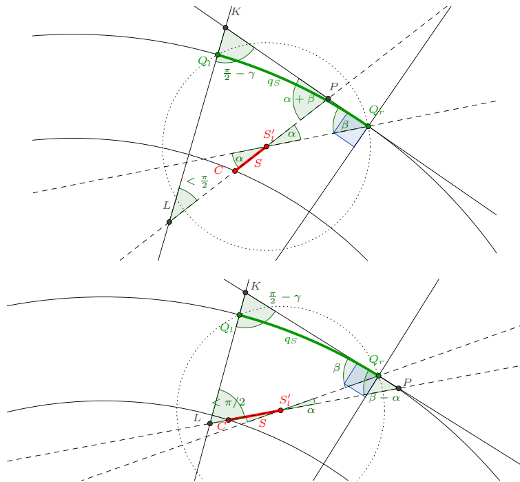
FIGURE 17. Picture to the case 3.1: ending component, n = 1, m = 1 .
