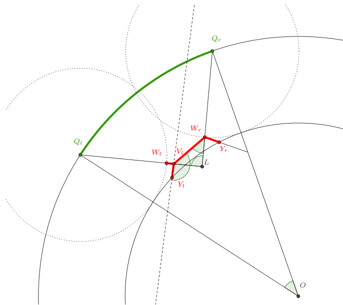
FIGURE 10. Picture to the case 3.1: middle component, n = 2, m = 2 .
