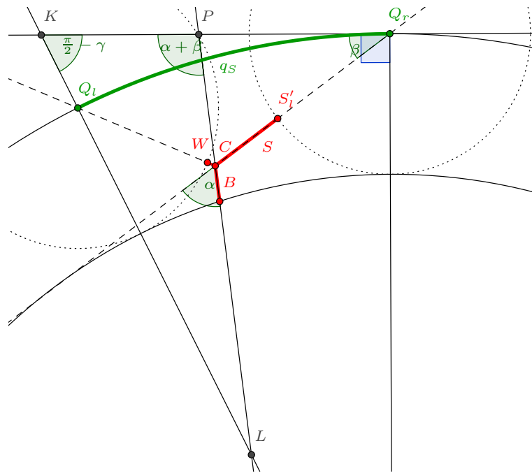
FIGURE 18. Picture to the case 3.1: ending component, n = 2, m = 1 .
