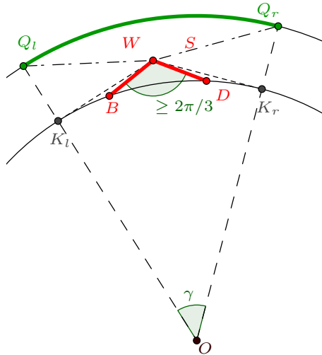
FIGURE 16. Picture to the case 3.1: middle component, m = 2, n = 1 .
