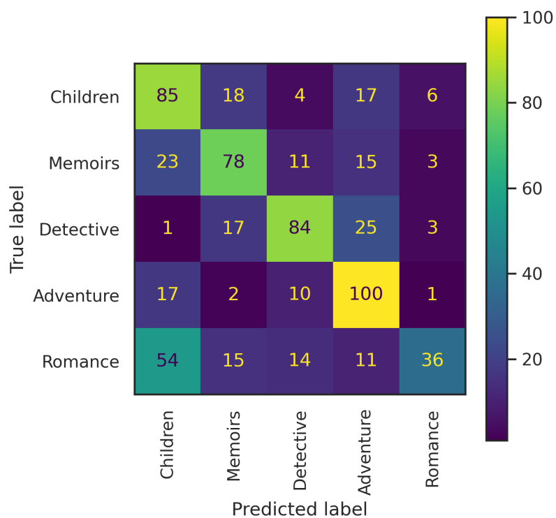
Figure 10: Confusion matrix for FAC features.
