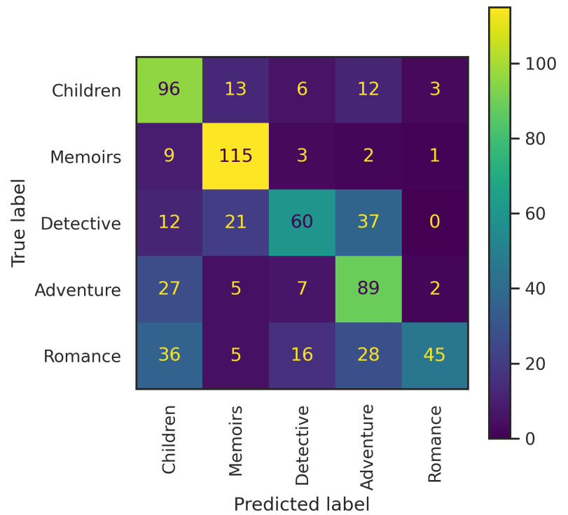
Figure 8: Confusion matrix for AGENT features.
