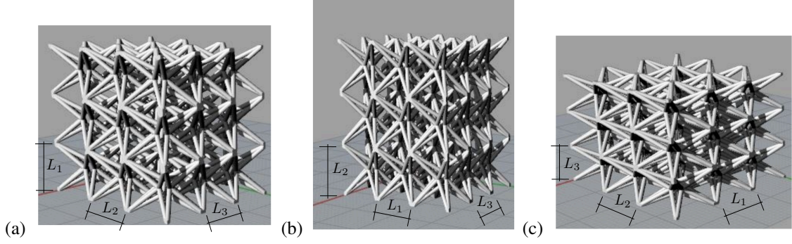
Figure 5: The three different configurations of the samples involved in the mechanical tests: (a) configuration C1, (b) configuration C2, (c) configuration C3
