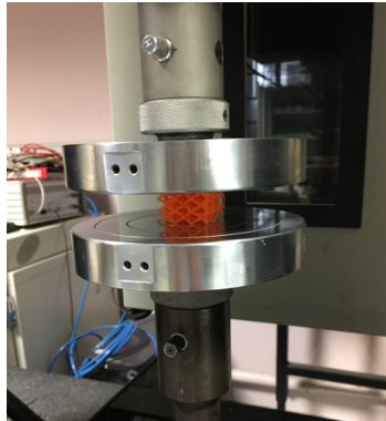
Figure 4: Polymeric samples: compression tests
