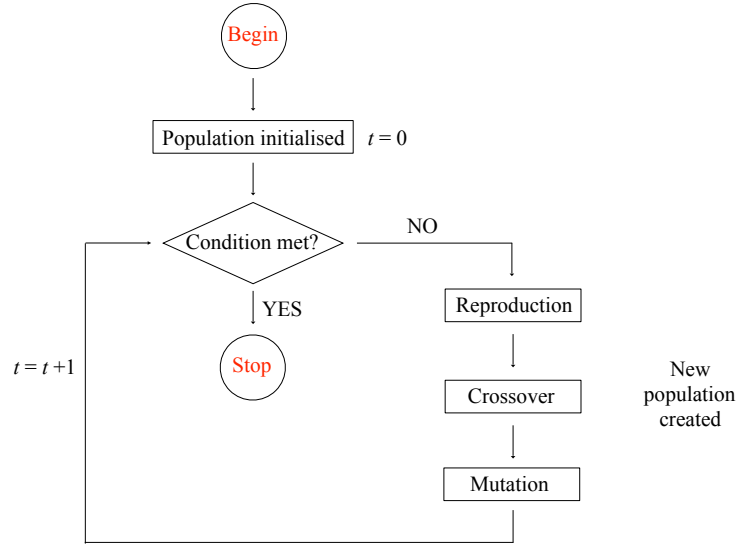
Figure 6: The genetic algorithm: working principle
