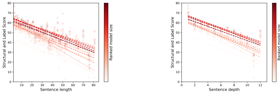
Figure 7: Comparative analysis of Polar Probe performance on the EN-EWT dataset as a function of sentence length (left) and sentence depth (right). The scores are shown across various model sizes (ranked by model size), with darker lines indicating larger models.
